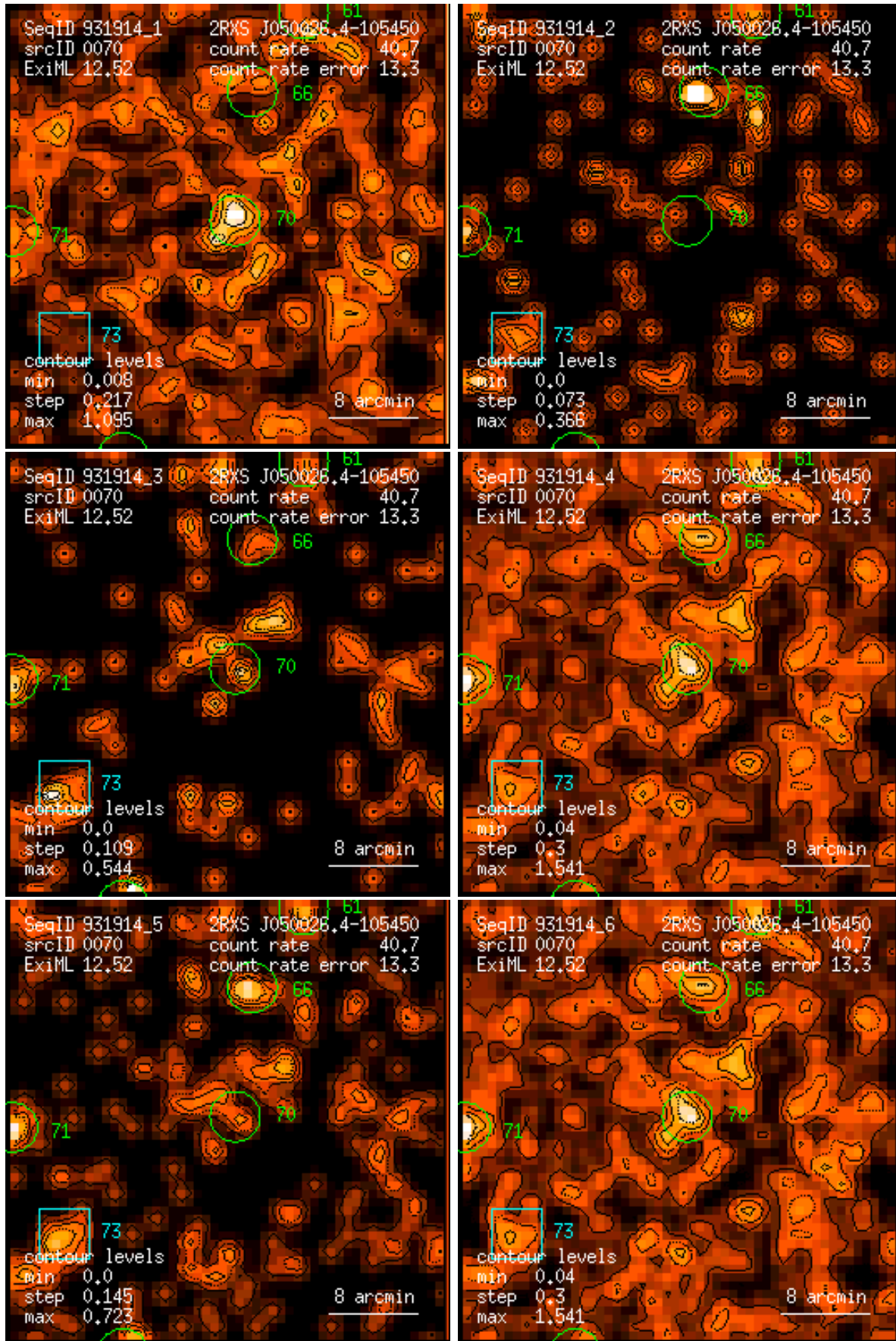
Figure 70: RASS 931914: detection 0070: band rate images, Gaussian filter: (1) PSPC channels 11 – 41, (2) 52 – 90, (3) 91 – 201, (4) 11 – 235, (5) 52 – 201, (6) 11 – 201. Broad band rates in counts/ks. Band rate contour levels in counts/ks/arcmin 2 .
