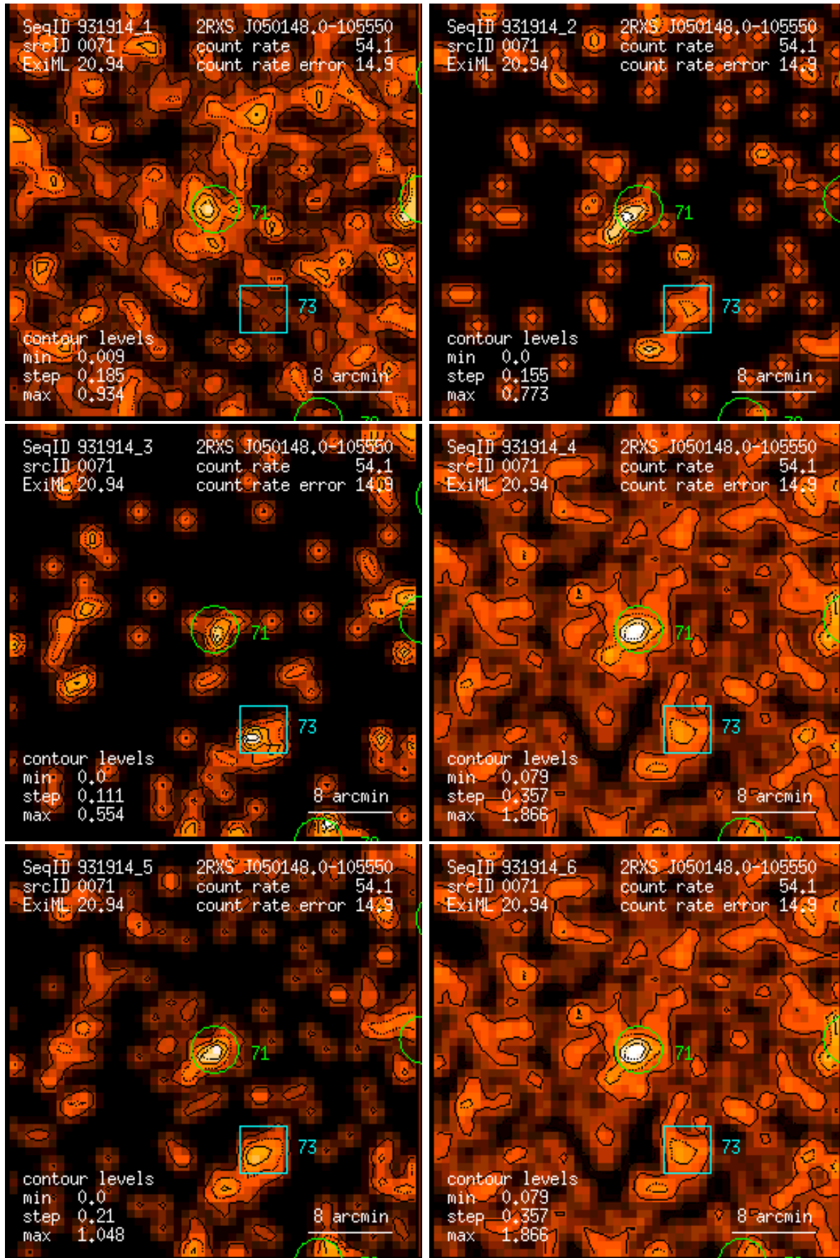
Figure 71: RASS 931914: detection 0071: band rate images, Gaussian filter: (1) PSPC channels 11 – 41, (2) 52 – 90, (3) 91 – 201, (4) 11 – 235, (5) 52 – 201, (6) 11 – 201. Broad band rates in counts/ks. Band rate contour levels in counts/ks/arcmin 2 .
