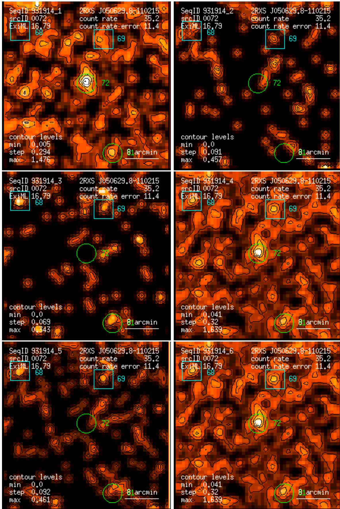
Figure 72: RASS 931914: detection 0072: band rate images, Gaussian filter: (1) PSPC channels 11 – 41, (2) 52 – 90, (3) 91 – 201, (4) 11 – 235, (5) 52 – 201, (6) 11 – 201. Broad band rates in counts/ks. Band rate contour levels in counts/ks/arcmin 2 .
