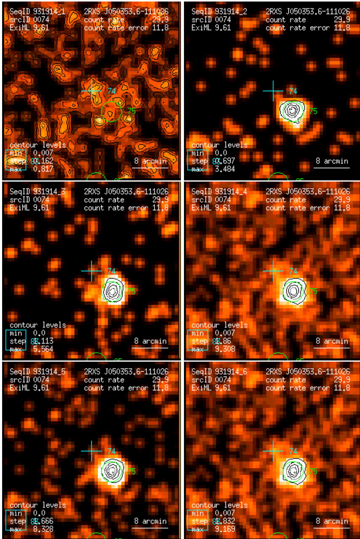
Figure 74: RASS 931914: detection 0074: band rate images, Gaussian filter: (1) PSPC channels 11 – 41, (2) 52 – 90, (3) 91 – 201, (4) 11 – 235, (5) 52 – 201, (6) 11 – 201. Broad band rates in counts/ks. Band rate contour levels in counts/ks/arcmin 2 .
