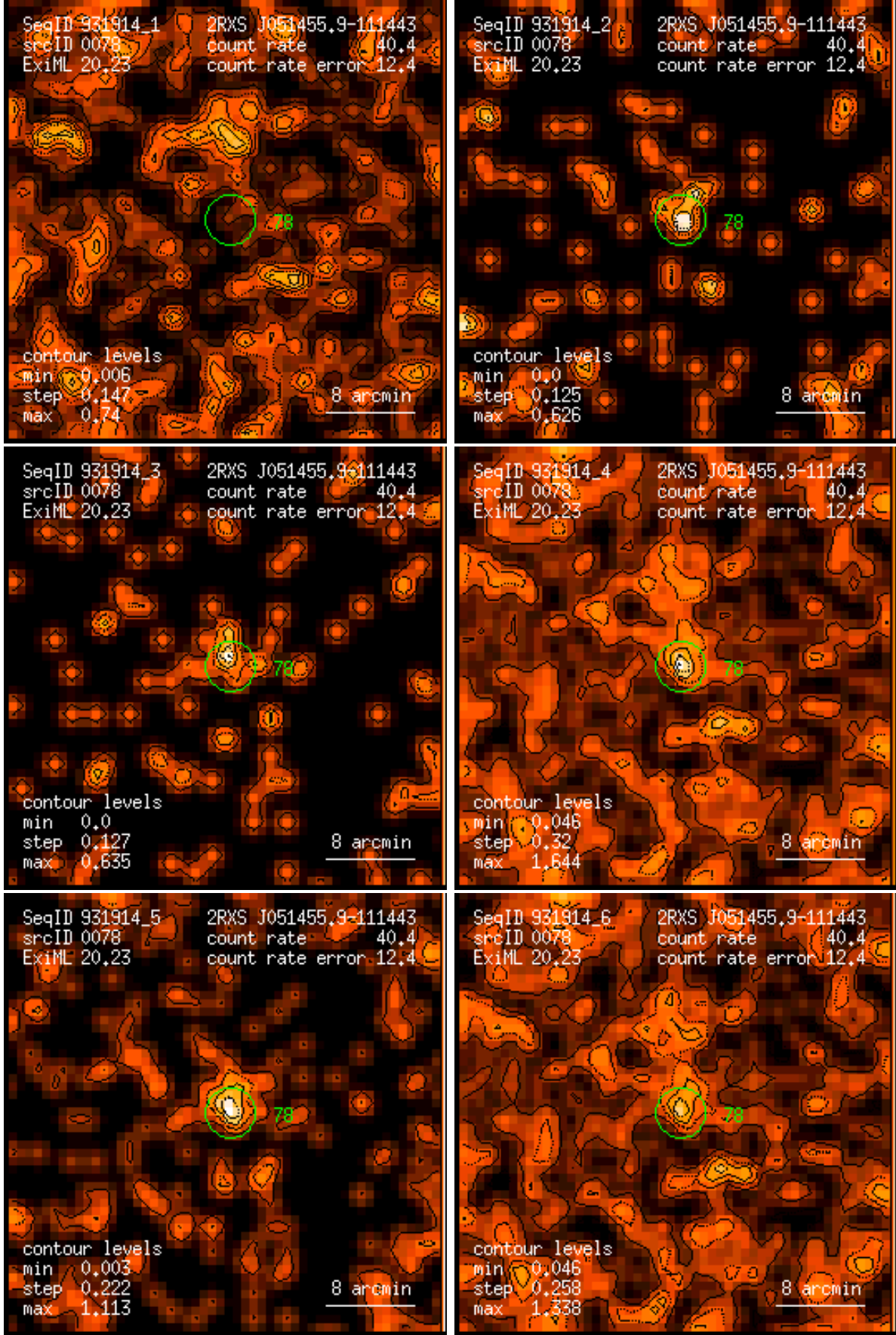
Figure 78: RASS 931914: detection 0078: band rate images, Gaussian filter: (1) PSPC channels 11 – 41, (2) 52 – 90, (3) 91 – 201, (4) 11 – 235, (5) 52 – 201, (6) 11 – 201. Broad band rates in counts/ks. Band rate contour levels in counts/ks/arcmin 2 .
