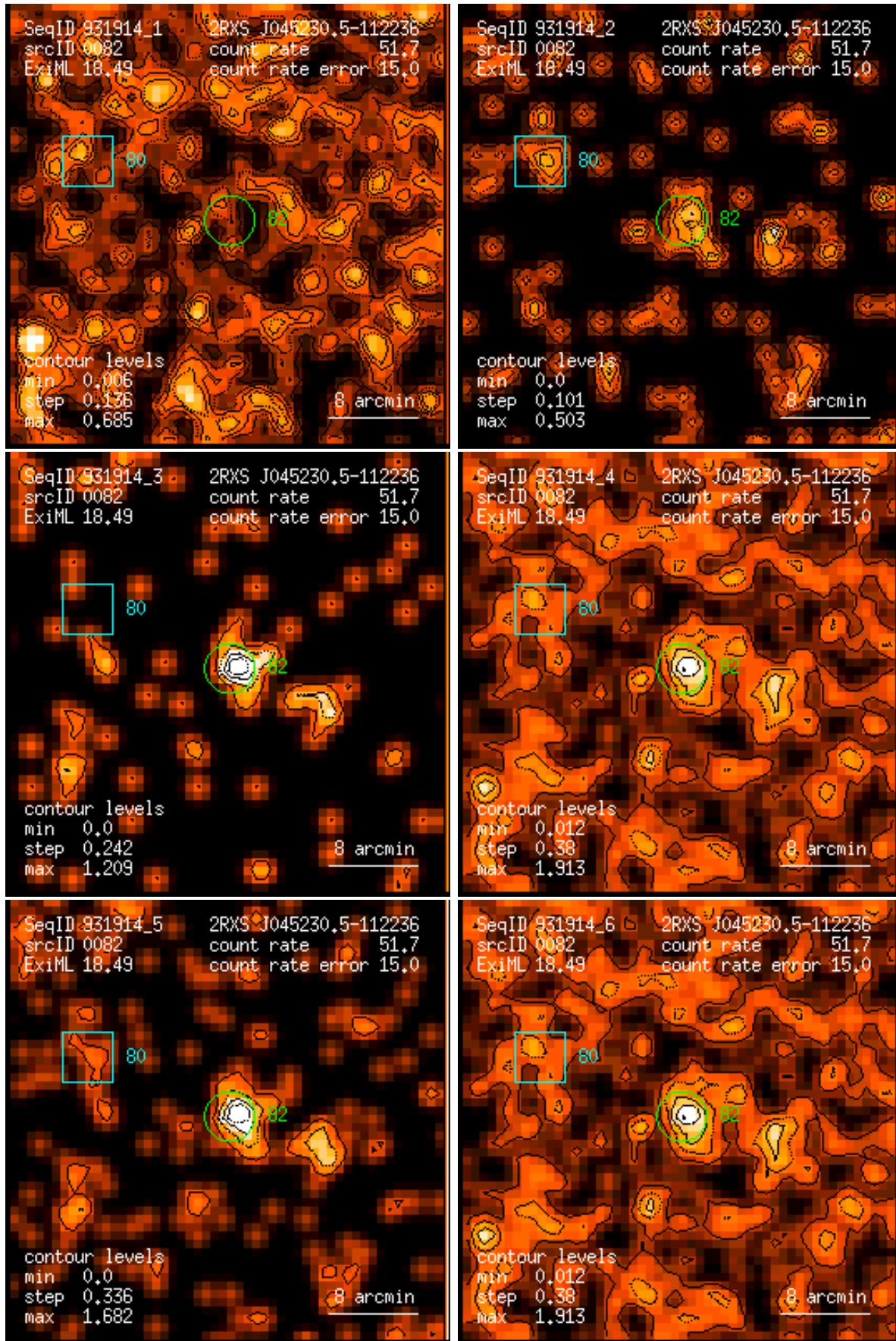
Figure 82: RASS 931914: detection 0082: band rate images, Gaussian filter: (1) PSPC channels 11 – 41, (2) 52 – 90, (3) 91 – 201, (4) 11 – 235, (5) 52 – 201, (6) 11 – 201. Broad band rates in counts/ks. Band rate contour levels in counts/ks/arcmin 2 .
