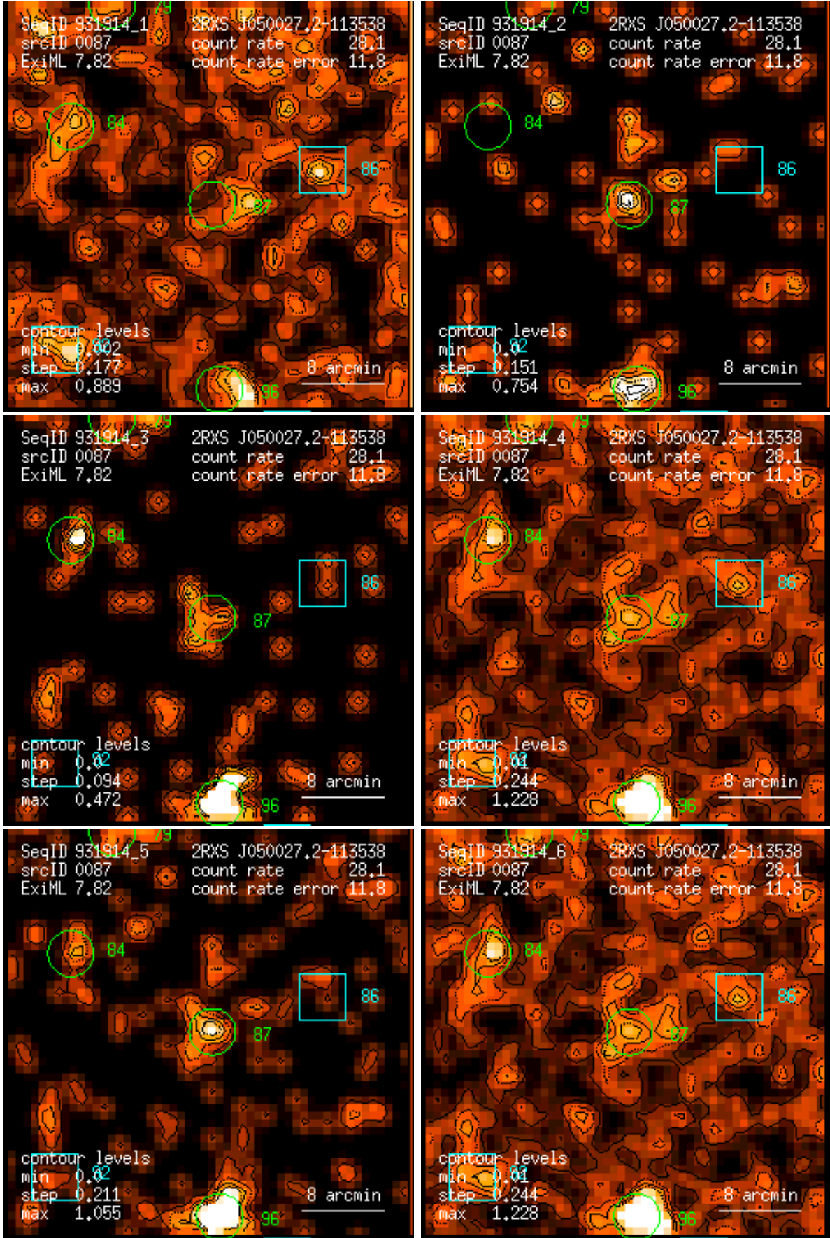
Figure 87: RASS 931914: detection 0087: band rate images, Gaussian filter: (1) PSPC channels 11 – 41, (2) 52 – 90, (3) 91 – 201, (4) 11 – 235, (5) 52 – 201, (6) 11 – 201. Broad band rates in counts/ks. Band rate contour levels in counts/ks/arcmin 2 .
