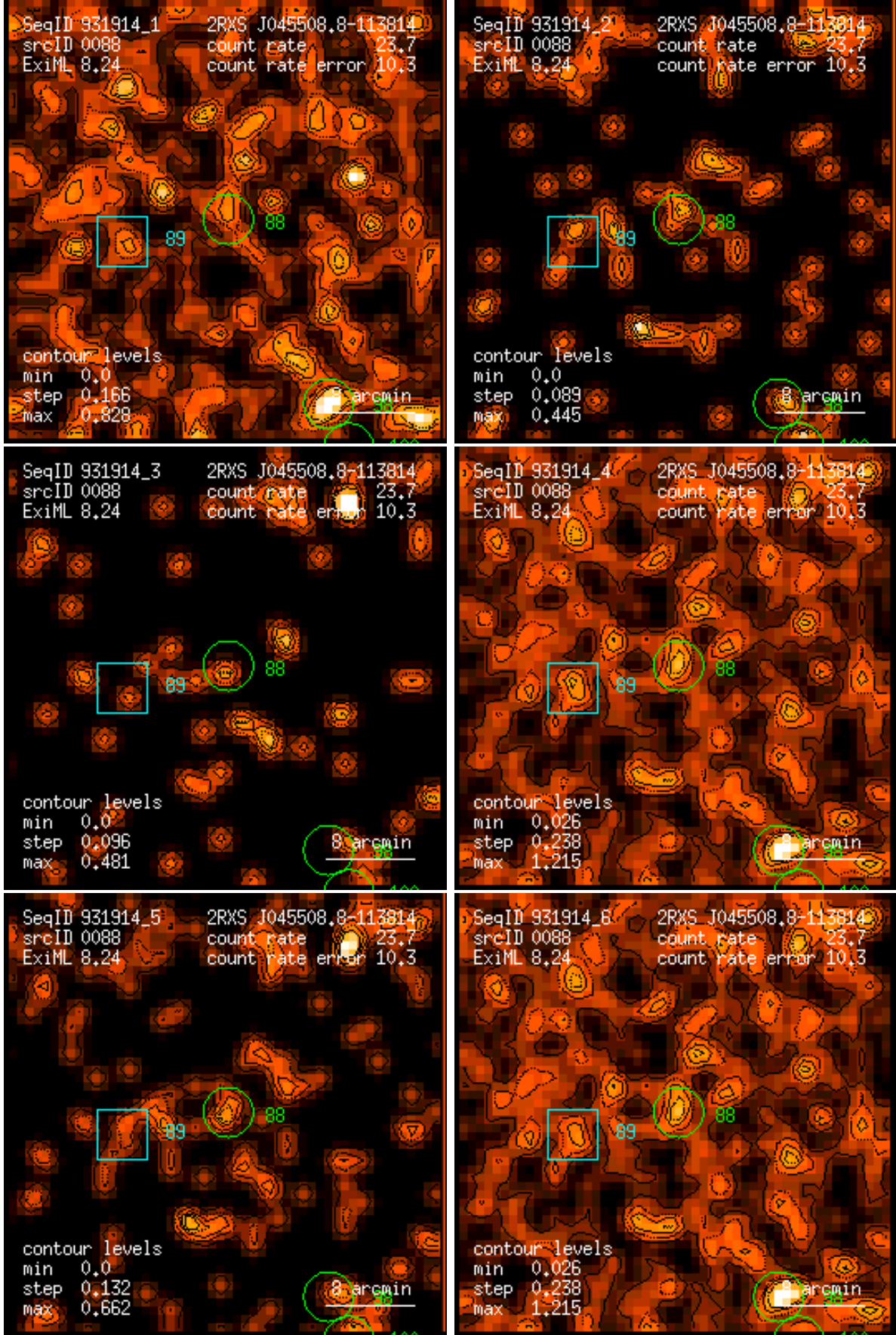
Figure 88: RASS 931914: detection 0088: band rate images, Gaussian filter: (1) PSPC channels 11 – 41, (2) 52 – 90, (3) 91 – 201, (4) 11 – 235, (5) 52 – 201, (6) 11 – 201. Broad band rates in counts/ks. Band rate contour levels in counts/ks/arcmin 2 .
