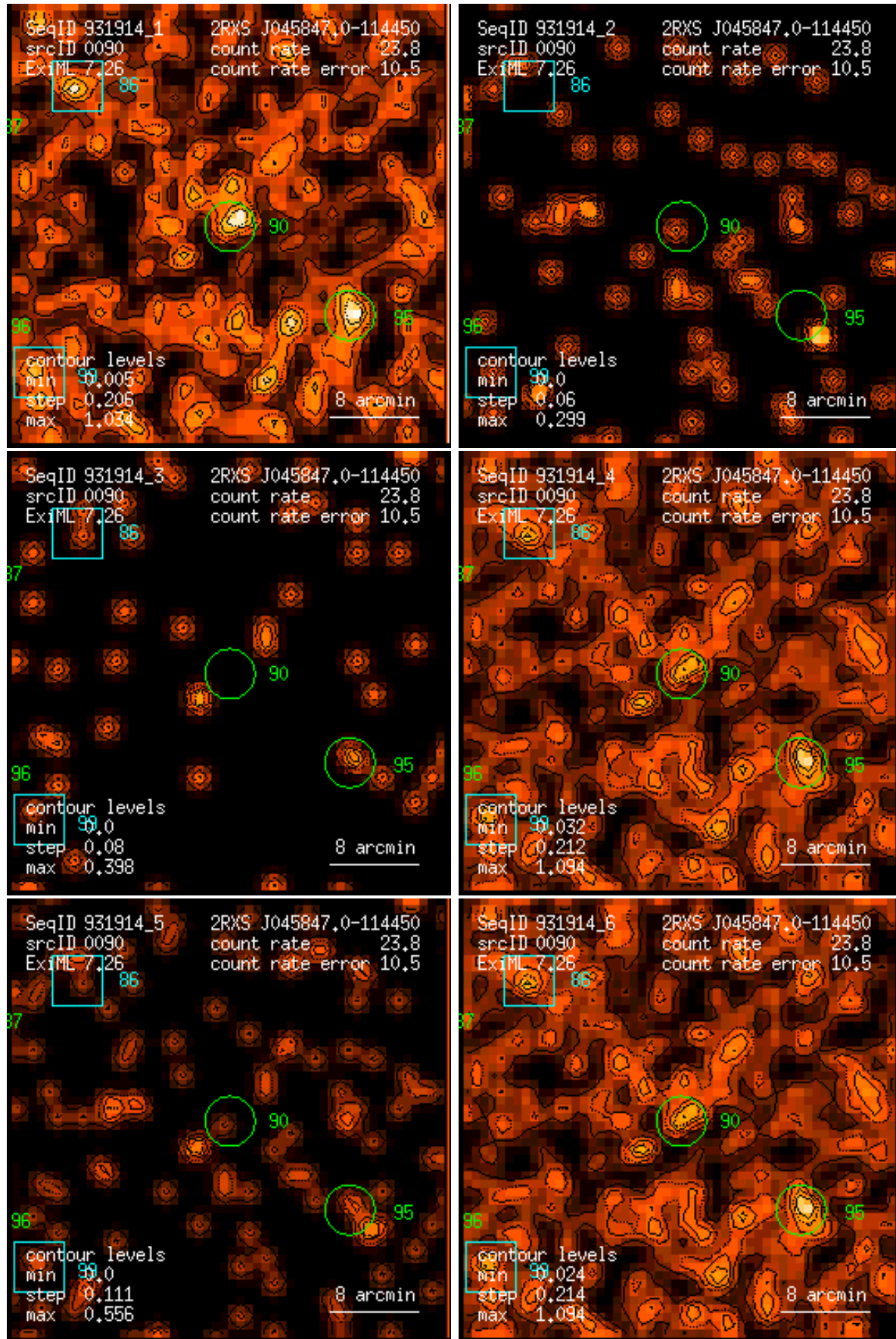
Figure 90: RASS 931914: detection 0090: band rate images, Gaussian filter: (1) PSPC channels 11 – 41, (2) 52 – 90, (3) 91 – 201, (4) 11 – 235, (5) 52 – 201, (6) 11 – 201. Broad band rates in counts/ks. Band rate contour levels in counts/ks/arcmin 2 .
