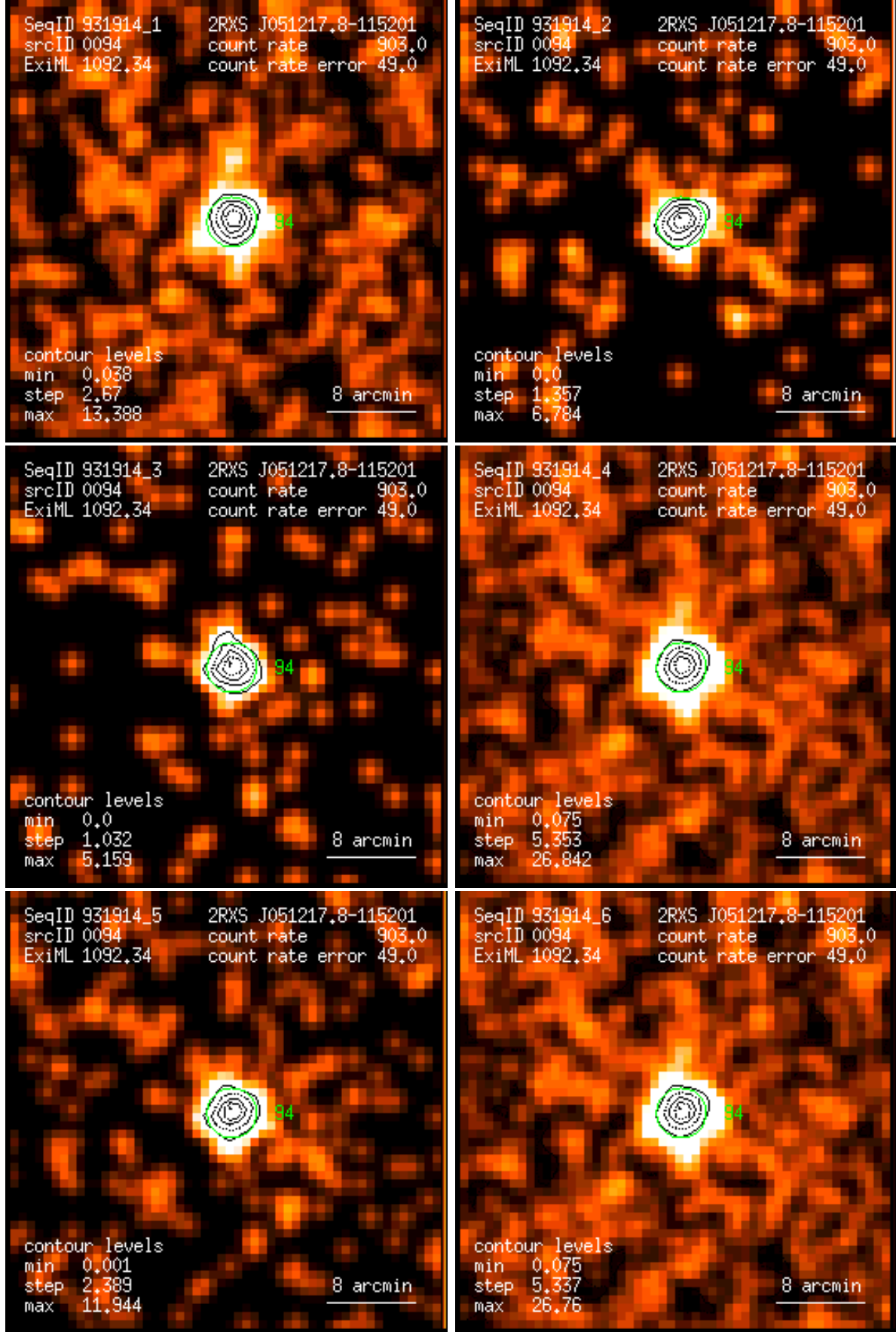
Figure 94: RASS 931914: detection 0094: band rate images, Gaussian filter: (1) PSPC channels 11 – 41, (2) 52 – 90, (3) 91 – 201, (4) 11 – 235, (5) 52 – 201, (6) 11 – 201. Broad band rates in counts/ks. Band rate contour levels in counts/ks/arcmin 2 .
