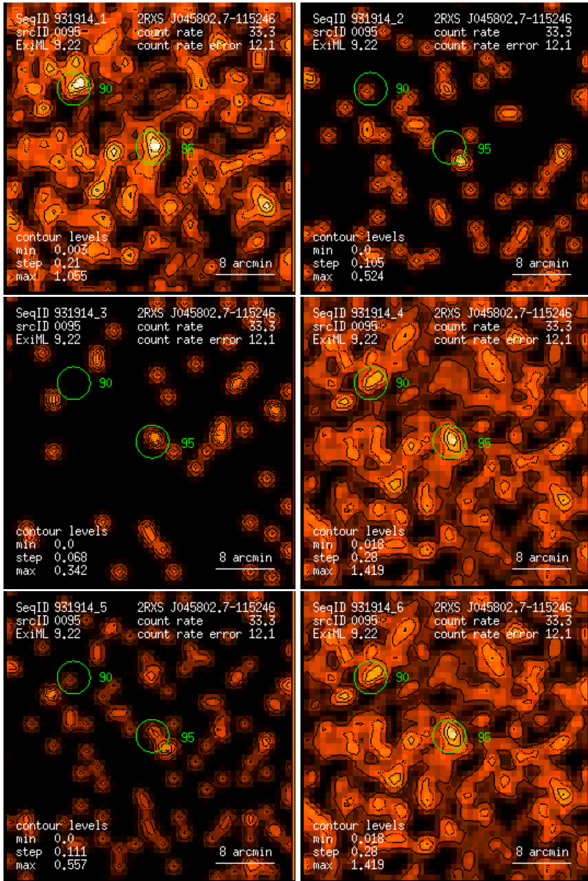
Figure 95: RASS 931914: detection 0095: band rate images, Gaussian filter: (1) PSPC channels 11 – 41, (2) 52 – 90, (3) 91 – 201, (4) 11 – 235, (5) 52 – 201, (6) 11 – 201. Broad band rates in counts/ks. Band rate contour levels in counts/ks/arcmin 2 .
