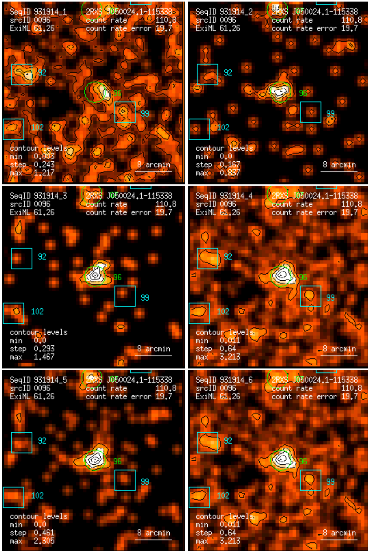
Figure 96: RASS 931914: detection 0096: band rate images, Gaussian filter: (1) PSPC channels 11 – 41, (2) 52 – 90, (3) 91 – 201, (4) 11 – 235, (5) 52 – 201, (6) 11 – 201. Broad band rates in counts/ks. Band rate contour levels in counts/ks/arcmin 2 .
