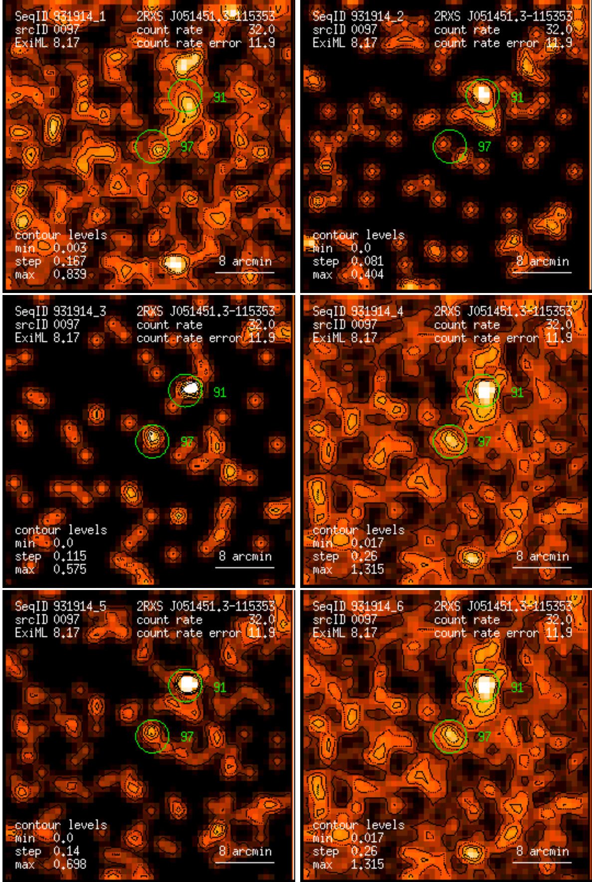
Figure 97: RASS 931914: detection 0097: band rate images, Gaussian filter: (1) PSPC channels 11 – 41, (2) 52 – 90, (3) 91 – 201, (4) 11 – 235, (5) 52 – 201, (6) 11 – 201. Broad band rates in counts/ks. Band rate contour levels in counts/ks/arcmin 2 .
