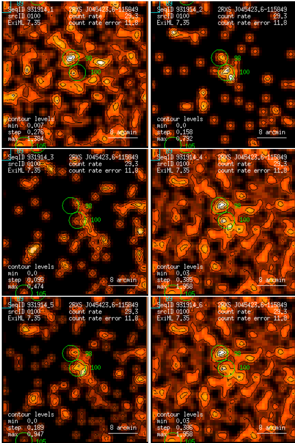
Figure 100: RASS 931914: detection 0100: band rate images, Gaussian filter: (1) PSPPC channels 11 – 41, (2) 52 – 90, (3) 91 – 201, (4) 11 – 235, (5) 52 – 201, (6) 11 – 201. Broad band rates in counts/ks. Band rate contour levels in counts/ks/arcmin 2 .
