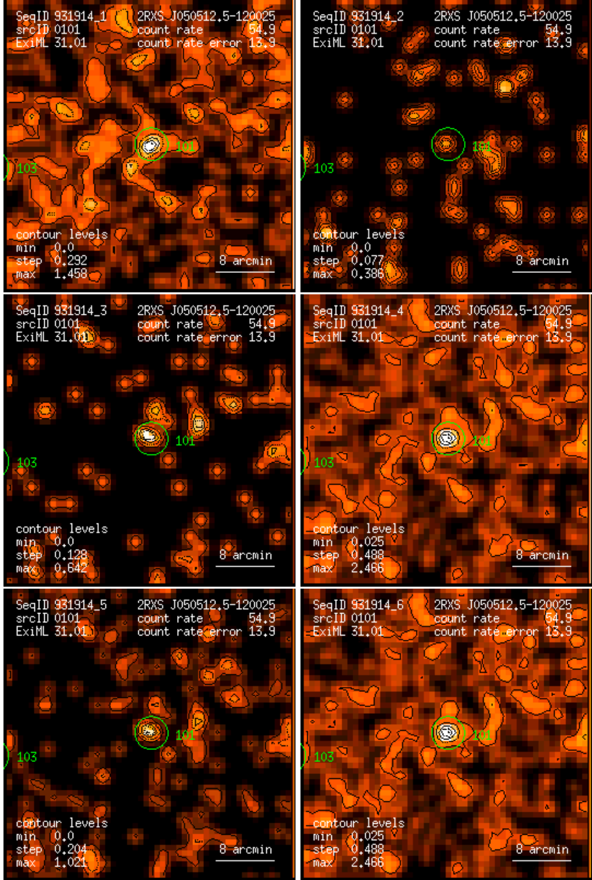
Figure 101: RASS 931914: detection 0101: band rate images, Gaussian filter: (1) PSPC channels 11 – 41, (2) 52 – 90, (3) 91 – 201, (4) 11 – 235, (5) 52 – 201, (6) 11 – 201. Broad band rates in counts/ks. Band rate contour levels in counts/ks/arcmin 2 .
