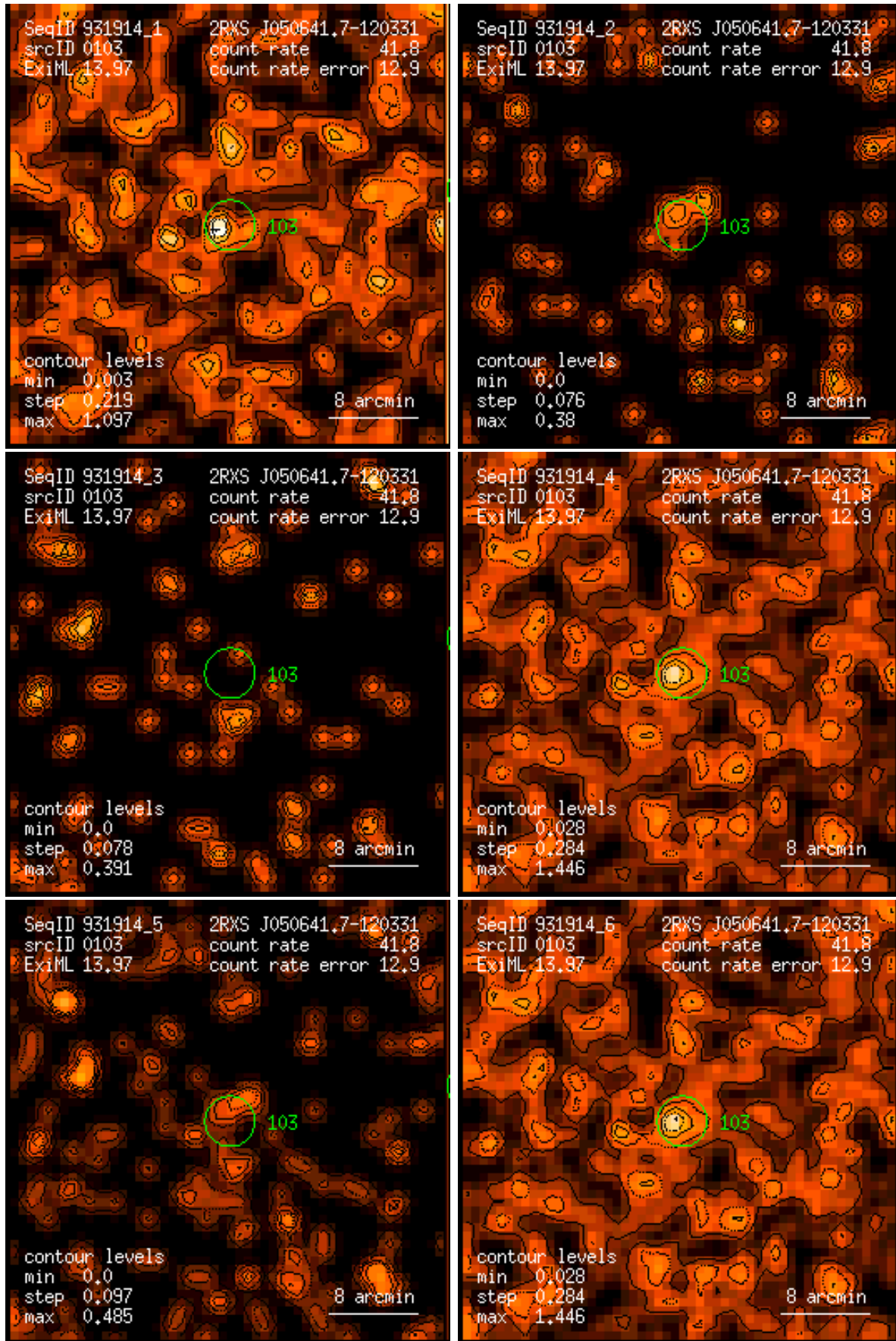
Figure 103: RASS 931914: detection 0103: band rate images, Gaussian filter: (1) PSPC channels 11 – 41, (2) 52 – 90, (3) 91 – 201, (4) 11 – 235, (5) 52 – 201, (6) 11 – 201. Broad band rates in counts/ks. Band rate contour levels in counts/ks/arcmin 2 .
