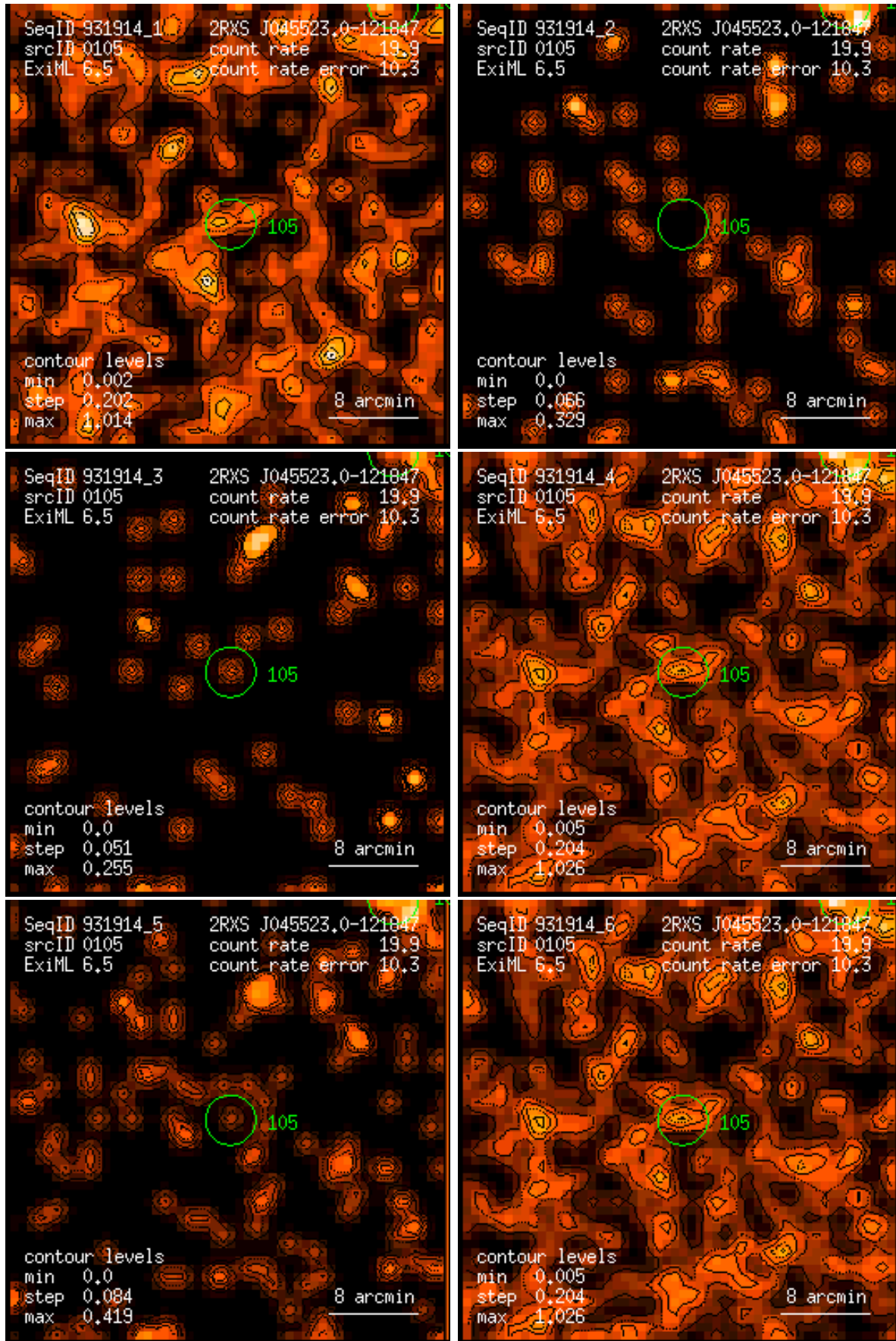
Figure 105: RASS 931914: detection 0105: band rate images, Gaussian filter: (1) PSPC channels 11 – 41, (2) 52 – 90, (3) 91 – 201, (4) 11 – 235, (5) 52 – 201, (6) 11 – 201. Broad band rates in counts/ks. Band rate contour levels in counts/ks/arcmin 2 .
