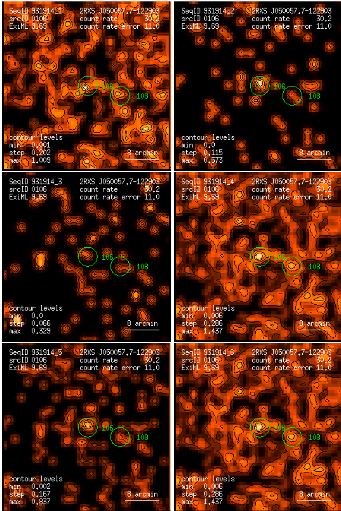
Figure 106: RASS 931914: detection 0106: band rate images, Gaussian filter: (1) PSPC channels 11 – 41, (2) 52 – 90, (3) 91 – 201, (4) 11 – 235, (5) 52 – 201, (6) 11 – 201. Broad band rates in counts/ks. Band rate contour levels in counts/ks/arcmin 2 .
