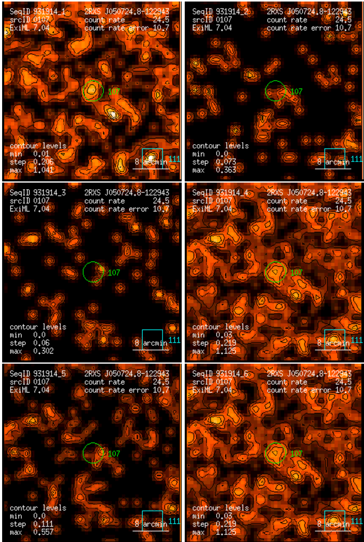
Figure 107: RASS 931914: detection 0107: band rate images, Gaussian filter: (1) PSPC channels 11 – 41, (2) 52 – 90, (3) 91 – 201, (4) 11 – 235, (5) 52 – 201, (6) 11 – 201. Broad band rates in counts/ks. Band rate contour levels in counts/ks/arcmin 2 .
