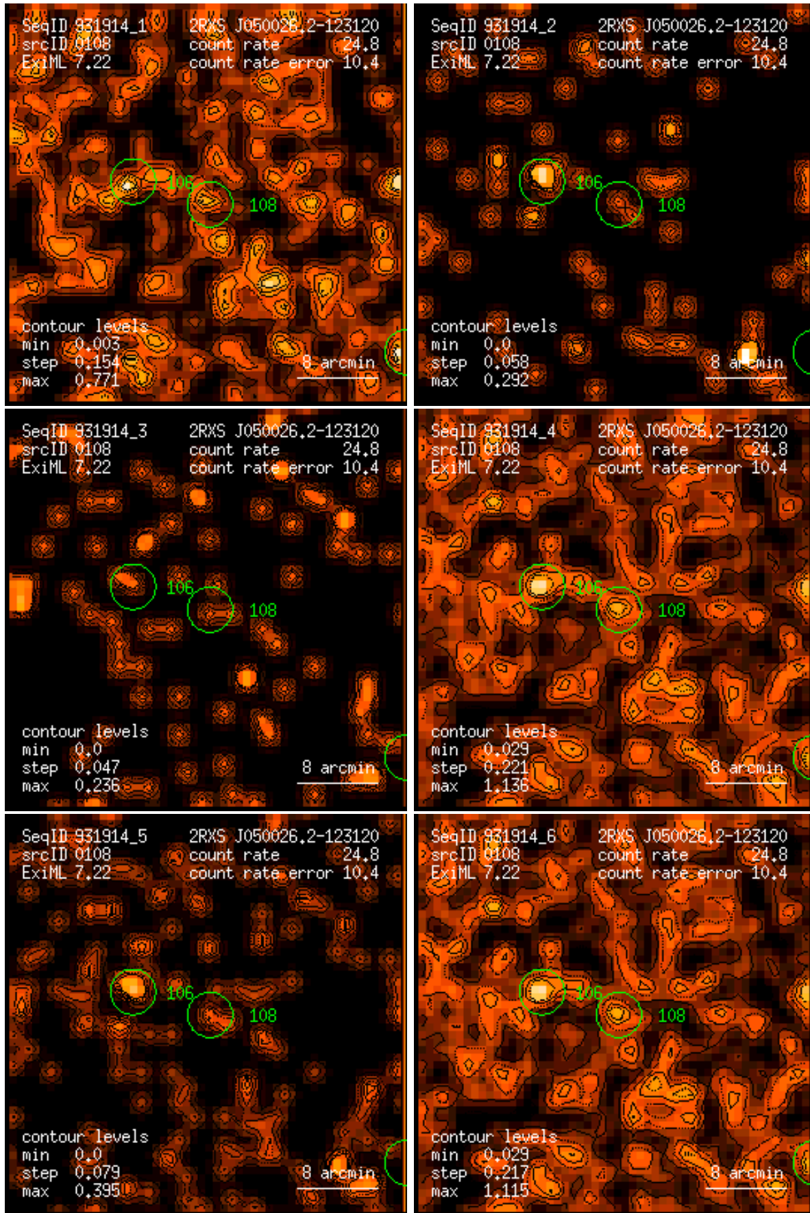
Figure 108: RASS 931914: detection 0108: band rate images, Gaussian filter: (1) PSPC channels 11 – 41, (2) 52 – 90, (3) 91 – 201, (4) 11 – 235, (5) 52 – 201, (6) 11 – 201. Broad band rates in counts/ks. Band rate contour levels in counts/ks/arcmin 2 .
