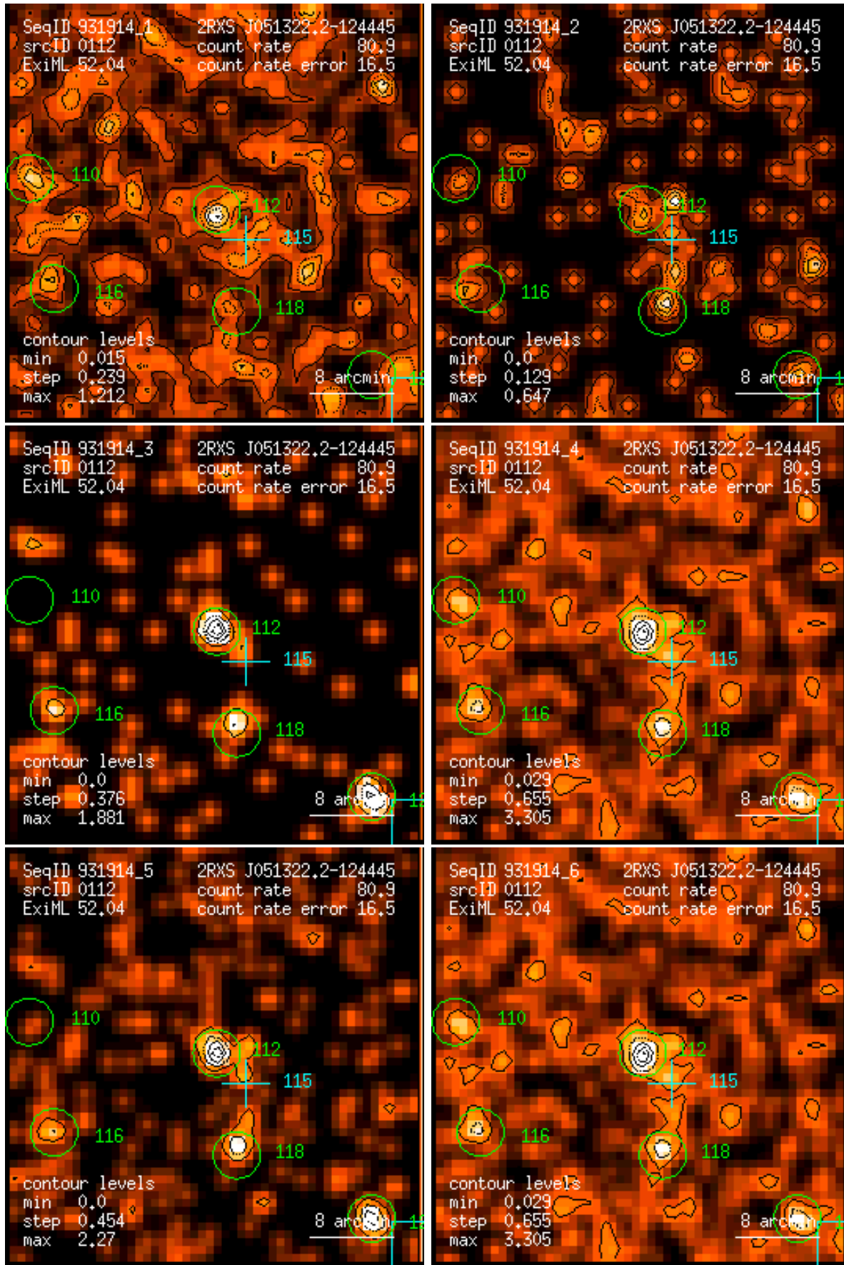
Figure 112: RASS 931914: detection 0112: band rate images, Gaussian filter: (1) PSPC channels 11 – 41, (2) 52 – 90, (3) 91 – 201, (4) 11 – 235, (5) 52 – 201, (6) 11 – 201. Broad band rates in counts/ks. Band rate contour levels in counts/ks/arcmin 2 .
