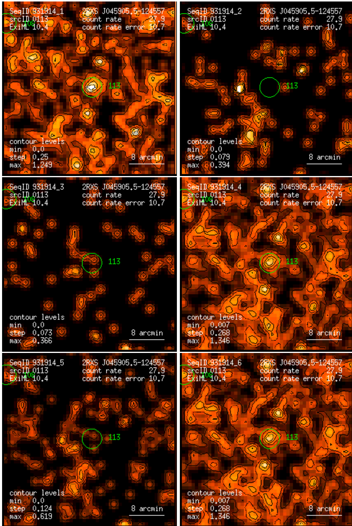
Figure 113: RASS 931914: detection 0113: band rate images, Gaussian filter: (1) PSPC channels 11 – 41, (2) 52 – 90, (3) 91 – 201, (4) 11 – 235, (5) 52 – 201, (6) 11 – 201. Broad band rates in counts/ks. Band rate contour levels in counts/ks/arcmin 2 .
