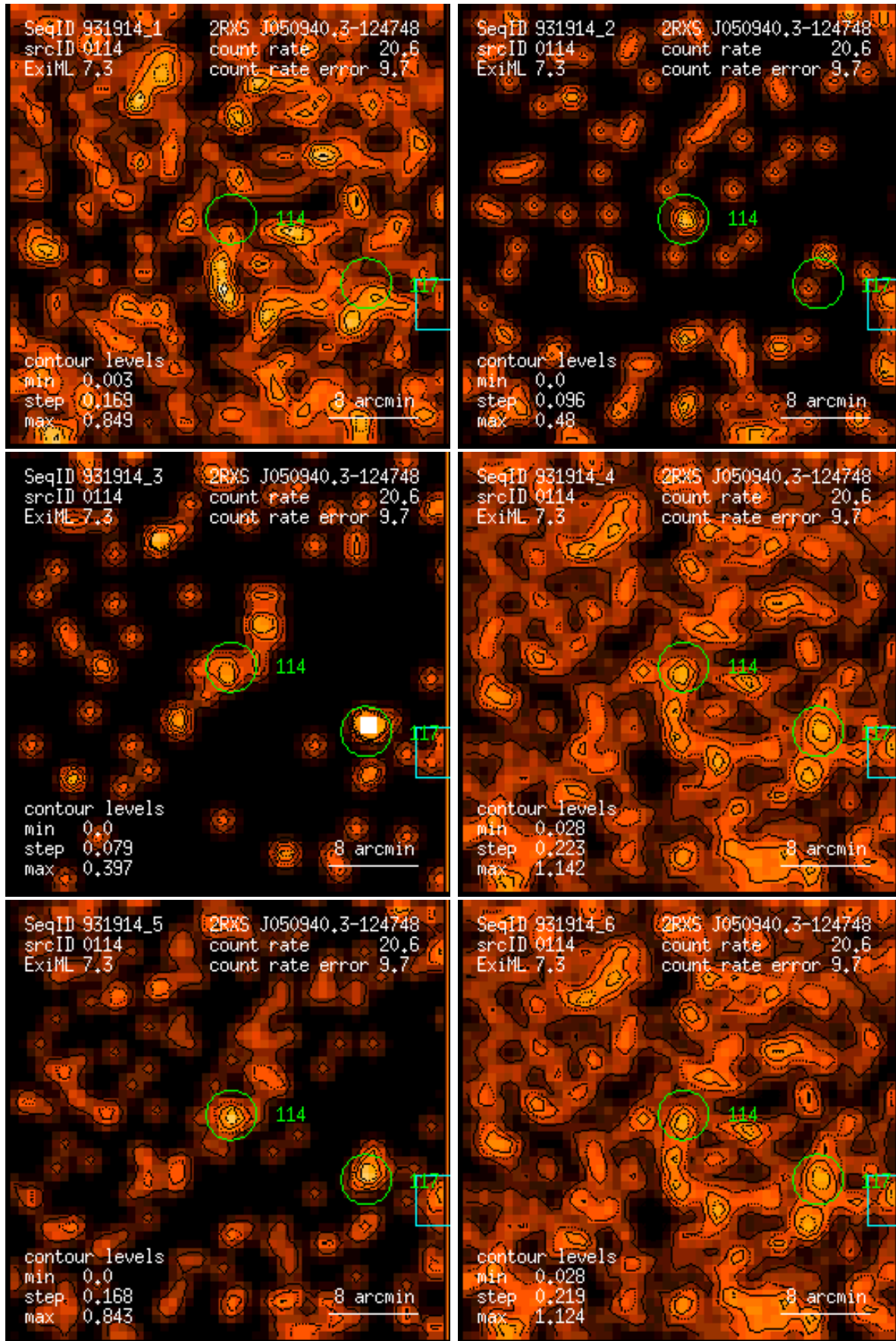
Figure 114: RASS 931914: detection 0114: band rate images, Gaussian filter: (1) PSPC channels 11 – 41, (2) 52 – 90, (3) 91 – 201, (4) 11 – 235, (5) 52 – 201, (6) 11 – 201. Broad band rates in counts/ks. Band rate contour levels in counts/ks/arcmin 2 .
