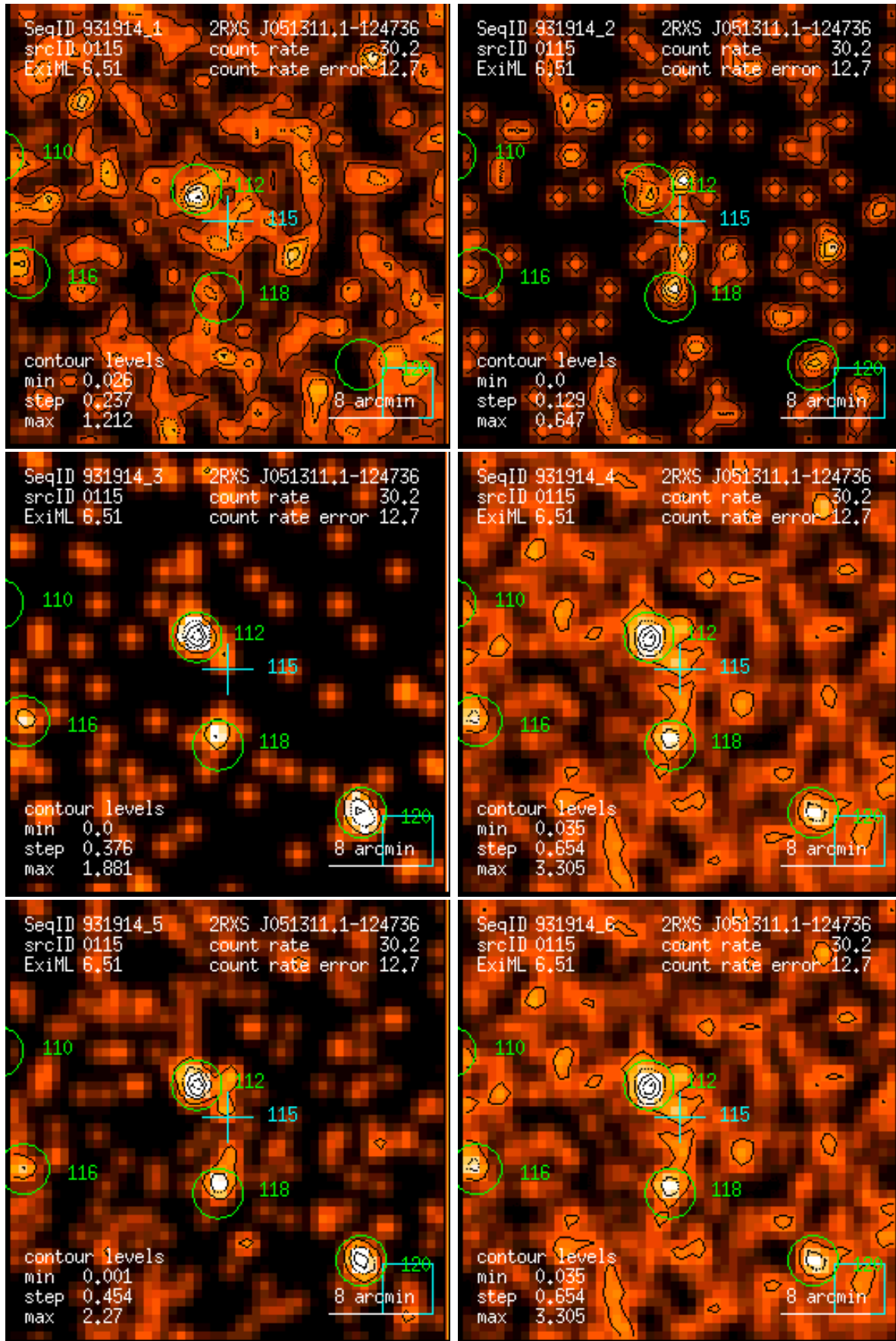
Figure 115: RASS 931914: detection 0115: band rate images, Gaussian filter: (1) PSPC channels 11 – 41, (2) 52 – 90, (3) 91 – 201, (4) 11 – 235, (5) 52 – 201, (6) 11 – 201. Broad band rates in counts/ks. Band rate contour levels in counts/ks/arcmin 2 .
