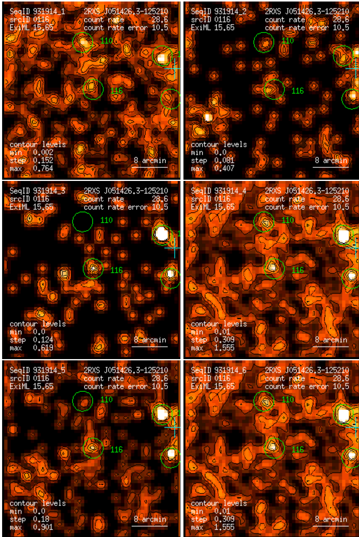
Figure 116: RASS 931914: detection 0116: band rate images, Gaussian filter: (1) PSPC channels 11 – 41, (2) 52 – 90, (3) 91 – 201, (4) 11 – 235, (5) 52 – 201, (6) 11 – 201. Broad band rates in counts/ks. Band rate contour levels in counts/ks/arcmin 2 .
