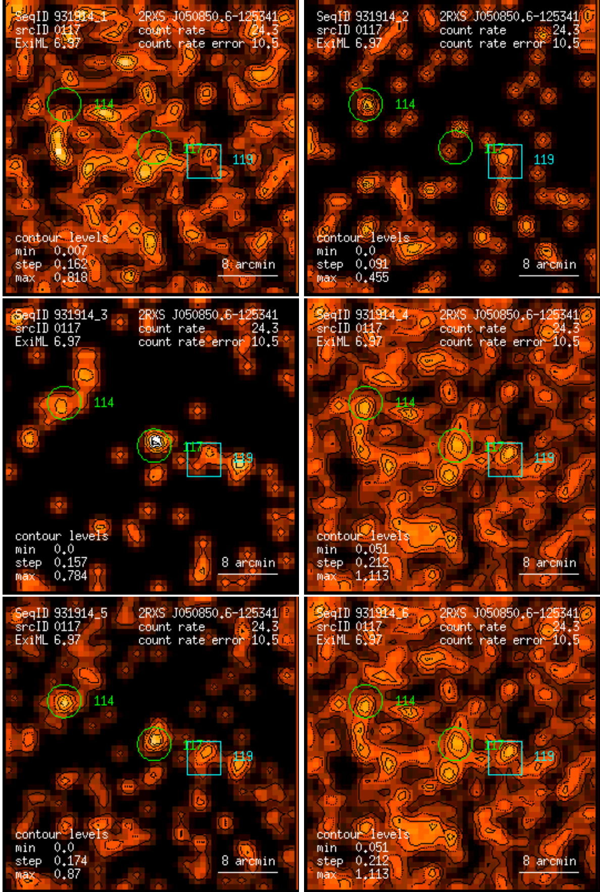
Figure 117: RASS 931914: detection 0117: band rate images, Gaussian filter: (1) PSPC channels 11 – 41, (2) 52 – 90, (3) 91 – 201, (4) 11 – 235, (5) 52 – 201, (6) 11 – 201. Broad band rates in counts/ks. Band rate contour levels in counts/ks/arcmin 2 .
