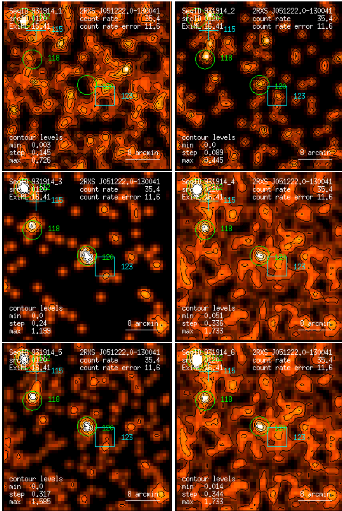
Figure 120: RASS 931914: detection 0120: band rate images, Gaussian filter: (1) PSPC channels 11 – 41, (2) 52 – 90, (3) 91 – 201, (4) 11 – 235, (5) 52 – 201, (6) 11 – 201. Broad band rates in counts/ks. Band rate contour levels in counts/ks/arcmin 2 .
