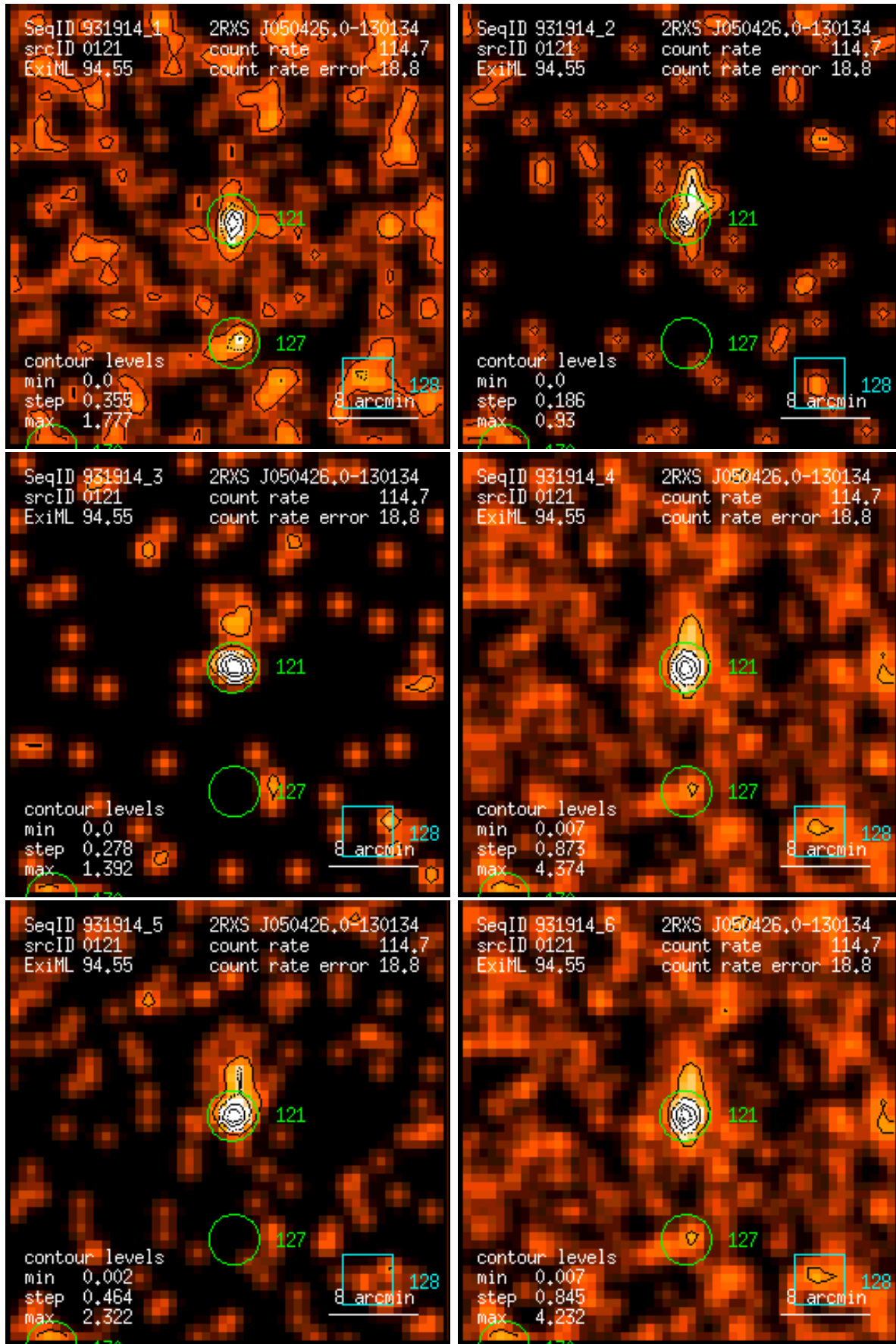
Figure 121: RASS 931914: detection 0121: band rate images, Gaussian filter: (1) PSPC channels 11 – 41, (2) 52 – 90, (3) 91 – 201, (4) 11 – 235, (5) 52 – 201, (6) 11 – 201. Broad band rates in counts/ks. Band rate contour levels in counts/ks/arcmin 2 .
