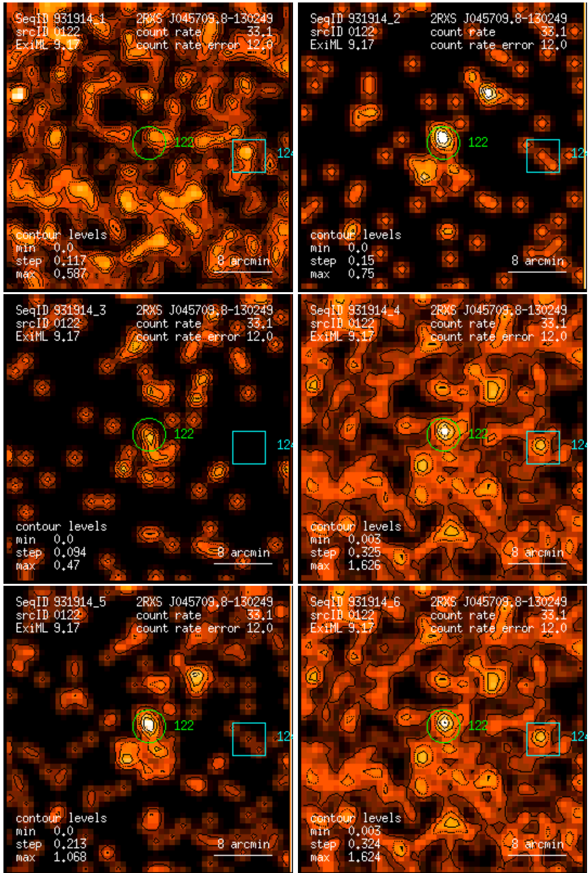
Figure 122: RASS 931914: detection 0122: band rate images, Gaussian filter: (1) PSPC channels 11 – 41, (2) 52 – 90, (3) 91 – 201, (4) 11 – 235, (5) 52 – 201, (6) 11 – 201. Broad band rates in counts/ks. Band rate contour levels in counts/ks/arcmin 2 .
