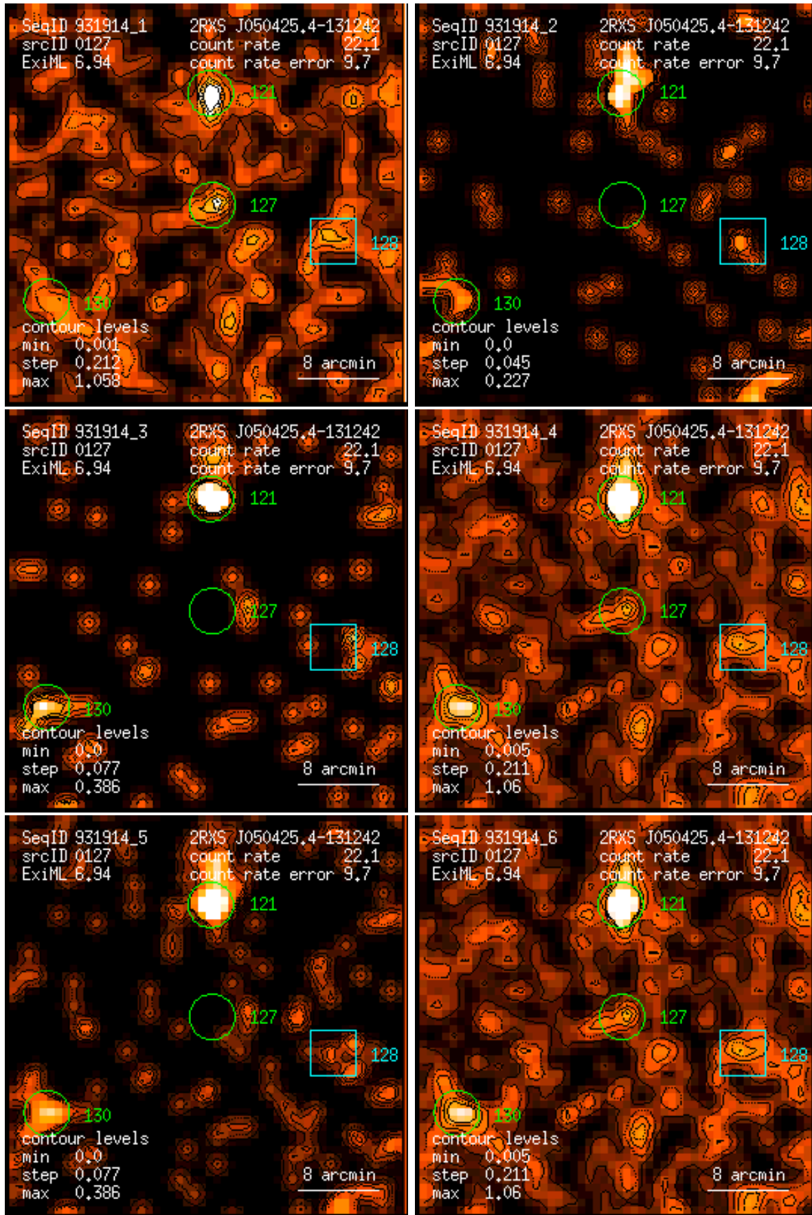
Figure 127: RASS 931914: detection 0127: band rate images, Gaussian filter: (1) PSPC channels 11 – 41, (2) 52 – 90, (3) 91 – 201, (4) 11 – 235, (5) 52 – 201, (6) 11 – 201. Broad band rates in counts/ks. Band rate contour levels in counts/ks/arcmin 2 .
