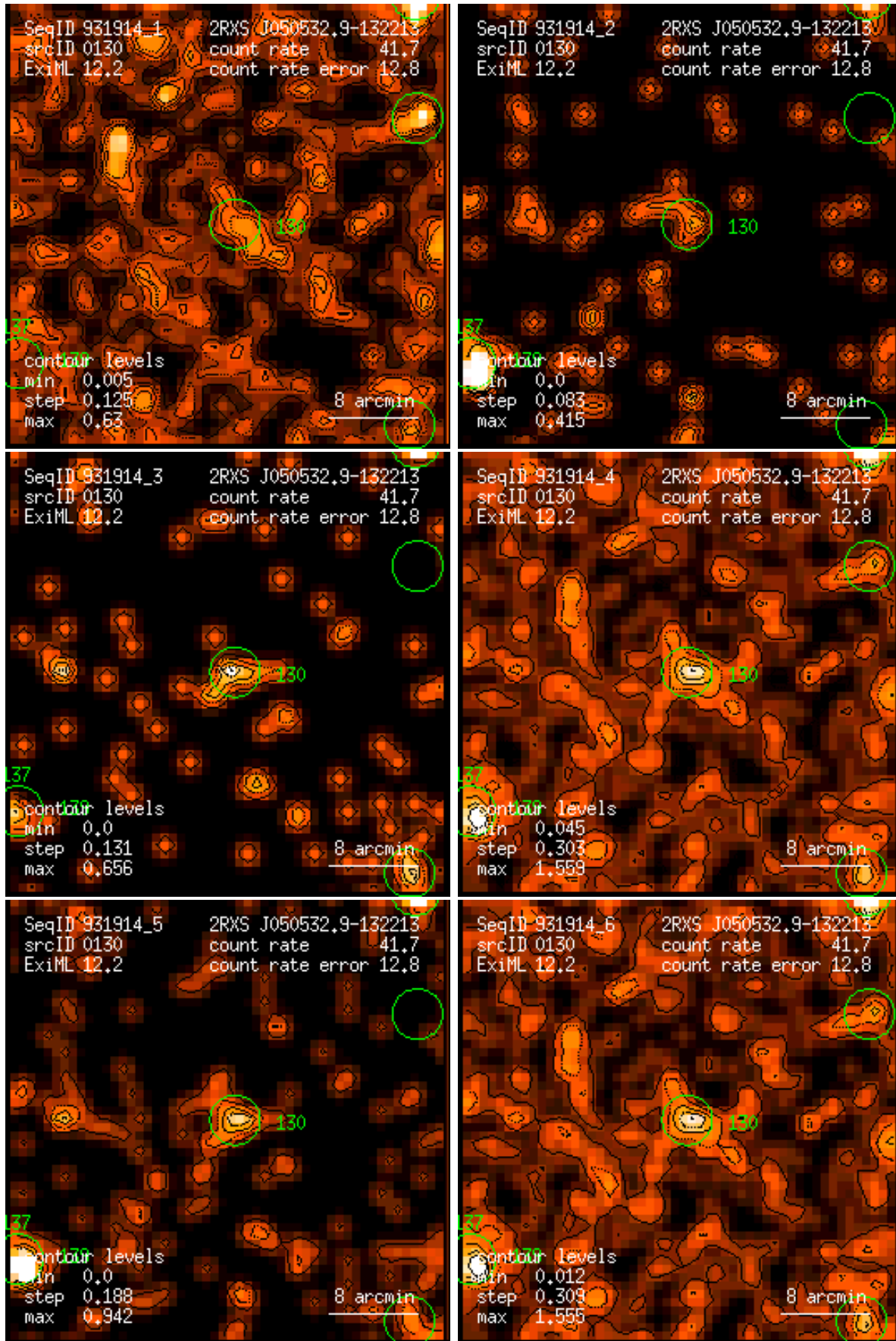
Figure 130: RASS 931914: detection 0130: band rate images, Gaussian filter: (1) PSPC channels 11 – 41, (2) 52 – 90, (3) 91 – 201, (4) 11 – 235, (5) 52 – 201, (6) 11 – 201. Broad band rates in counts/ks. Band rate contour levels in counts/ks/arcmin 2 .
