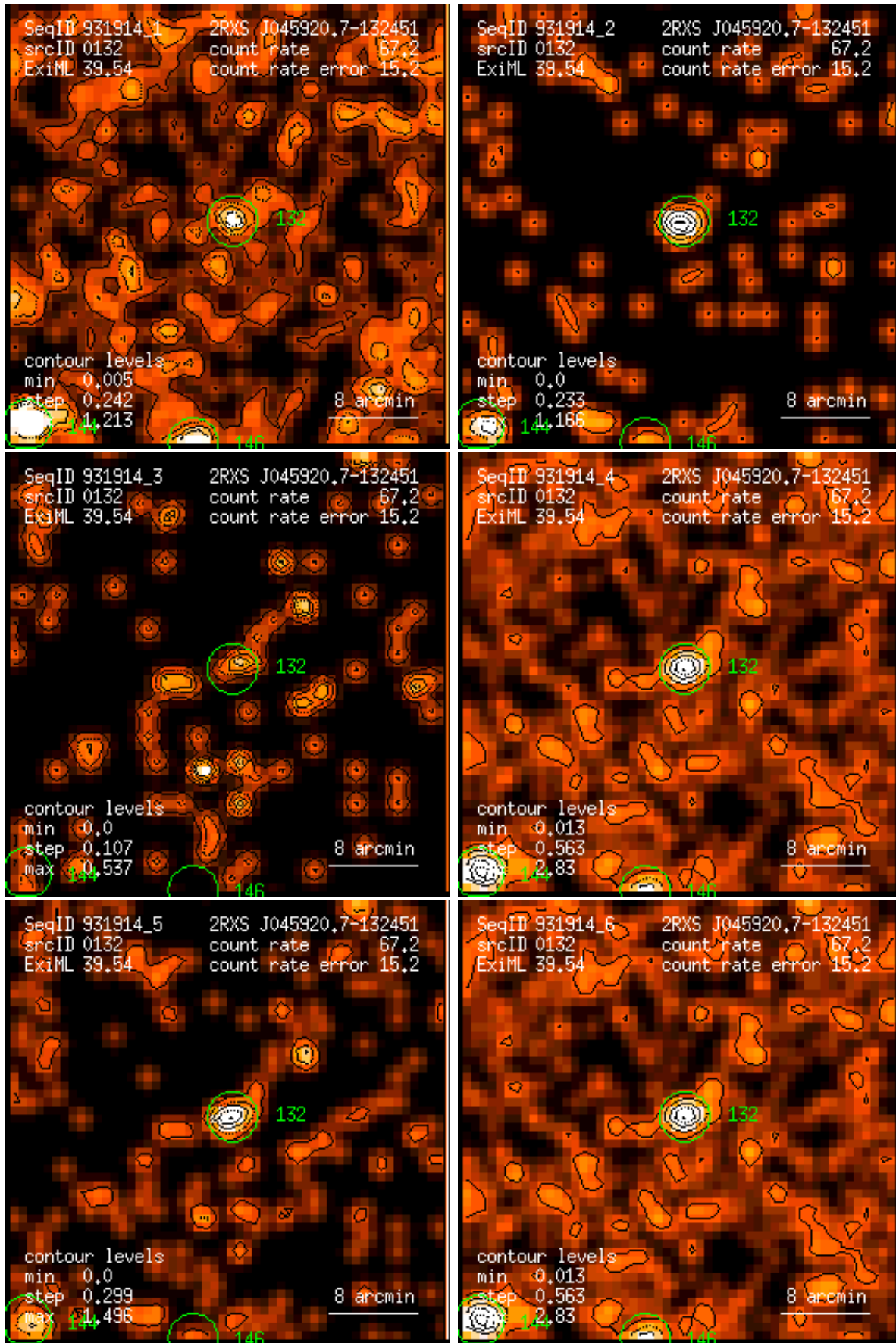
Figure 132: RASS 931914: detection 0132: band rate images, Gaussian filter: (1) PSPC channels 11 – 41, (2) 52 – 90, (3) 91 – 201, (4) 11 – 235, (5) 52 – 201, (6) 11 – 201. Broad band rates in counts/ks. Band rate contour levels in counts/ks/arcmin 2 .
