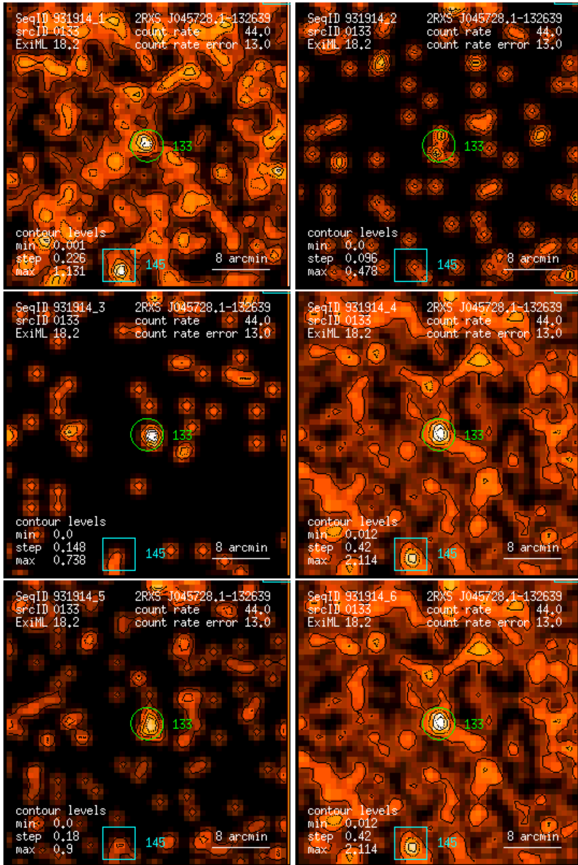
Figure 133: RASS 931914: detection 0133: band rate images, Gaussian filter: (1) PSPC channels 11 – 41, (2) 52 – 90, (3) 91 – 201, (4) 11 – 235, (5) 52 – 201, (6) 11 – 201. Broad band rates in counts/ks. Band rate contour levels in counts/ks/arcmin 2 .
