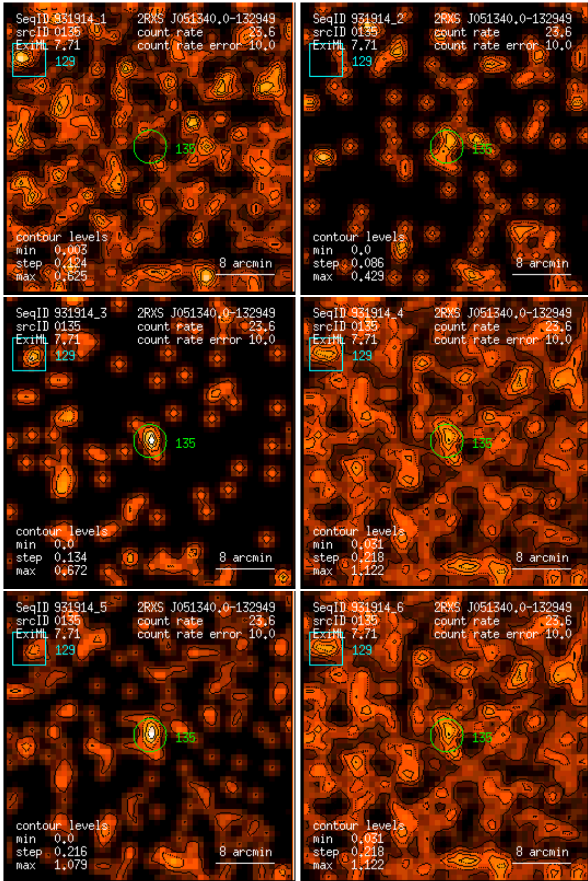
Figure 135: RASS 931914: detection 0135: band rate images, Gaussian filter: (1) PSPC channels 11 – 41, (2) 52 – 90, (3) 91 – 201, (4) 11 – 235, (5) 52 – 201, (6) 11 – 201. Broad band rates in counts/ks. Band rate contour levels in counts/ks/arcmin 2 .
