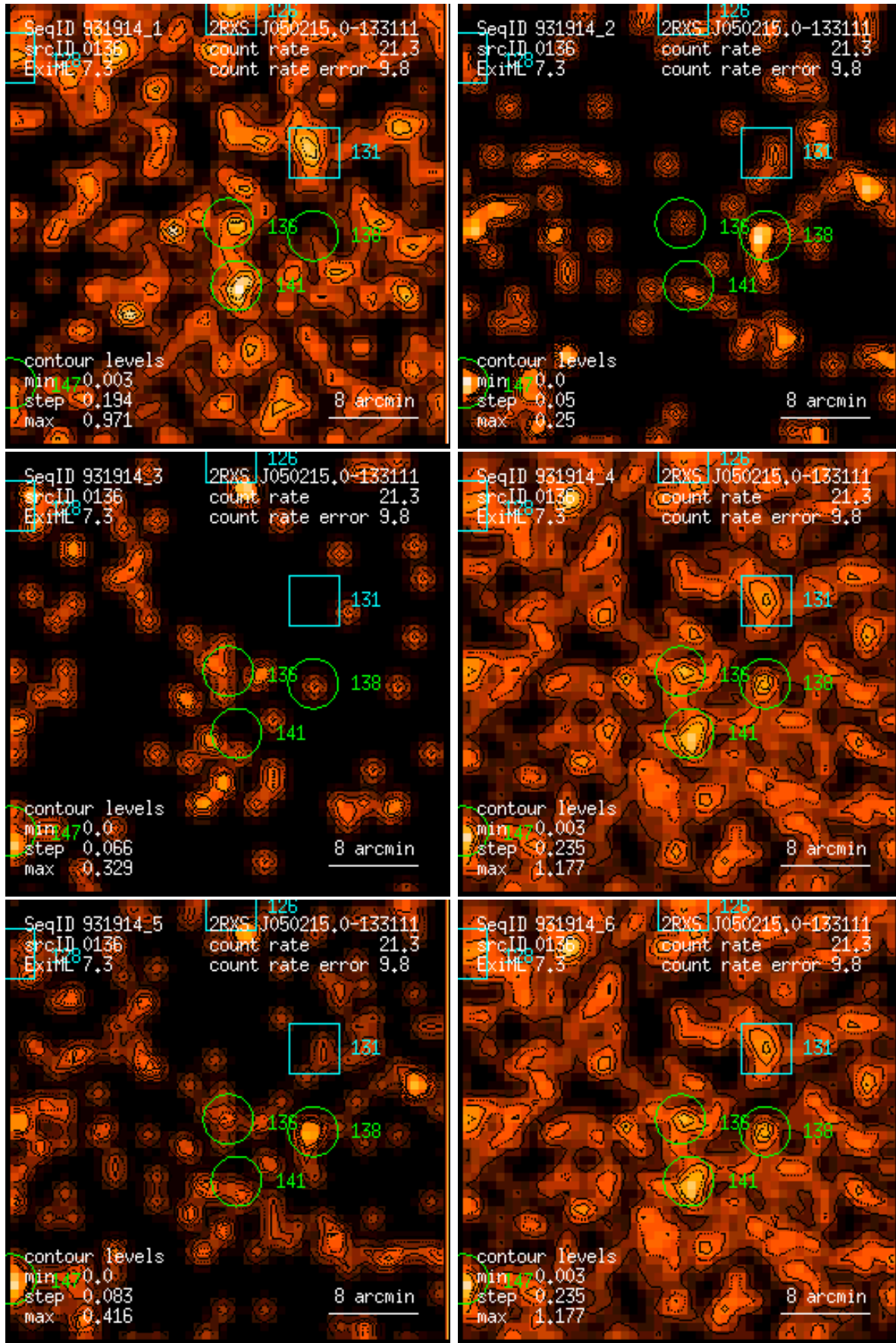
Figure 136: RASS 931914: detection 0136: band rate images, Gaussian filter: (1) PSPC channels 11 – 41, (2) 52 – 90, (3) 91 – 201, (4) 11 – 235, (5) 52 – 201, (6) 11 – 201. Broad band rates in counts/ks. Band rate contour levels in counts/ks/arcmin 2 .
