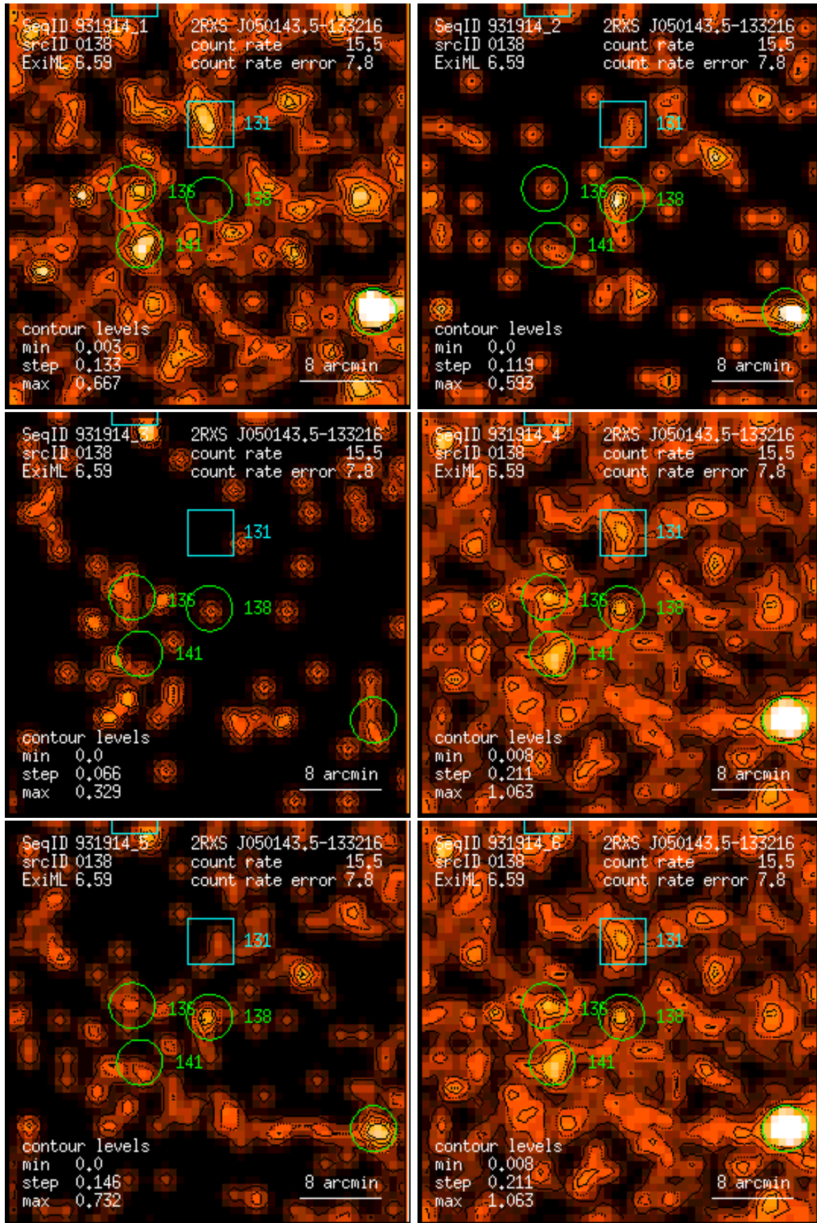
Figure 138: RASS 931914: detection 0138: band rate images, Gaussian filter: (1) PSPC channels 11 – 41, (2) 52 – 90, (3) 91 – 201, (4) 11 – 235, (5) 52 – 201, (6) 11 – 201. Broad band rates in counts/ks. Band rate contour levels in counts/ks/arcmin 2 .
