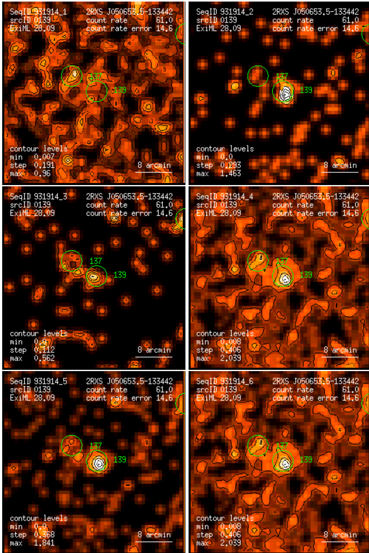
Figure 139: RASS 931914: detection 0139: band rate images, Gaussian filter: (1) PSPC channels 11 – 41, (2) 52 – 90, (3) 91 – 201, (4) 11 – 235, (5) 52 – 201, (6) 11 – 201. Broad band rates in counts/ks. Band rate contour levels in counts/ks/arcmin 2 .
