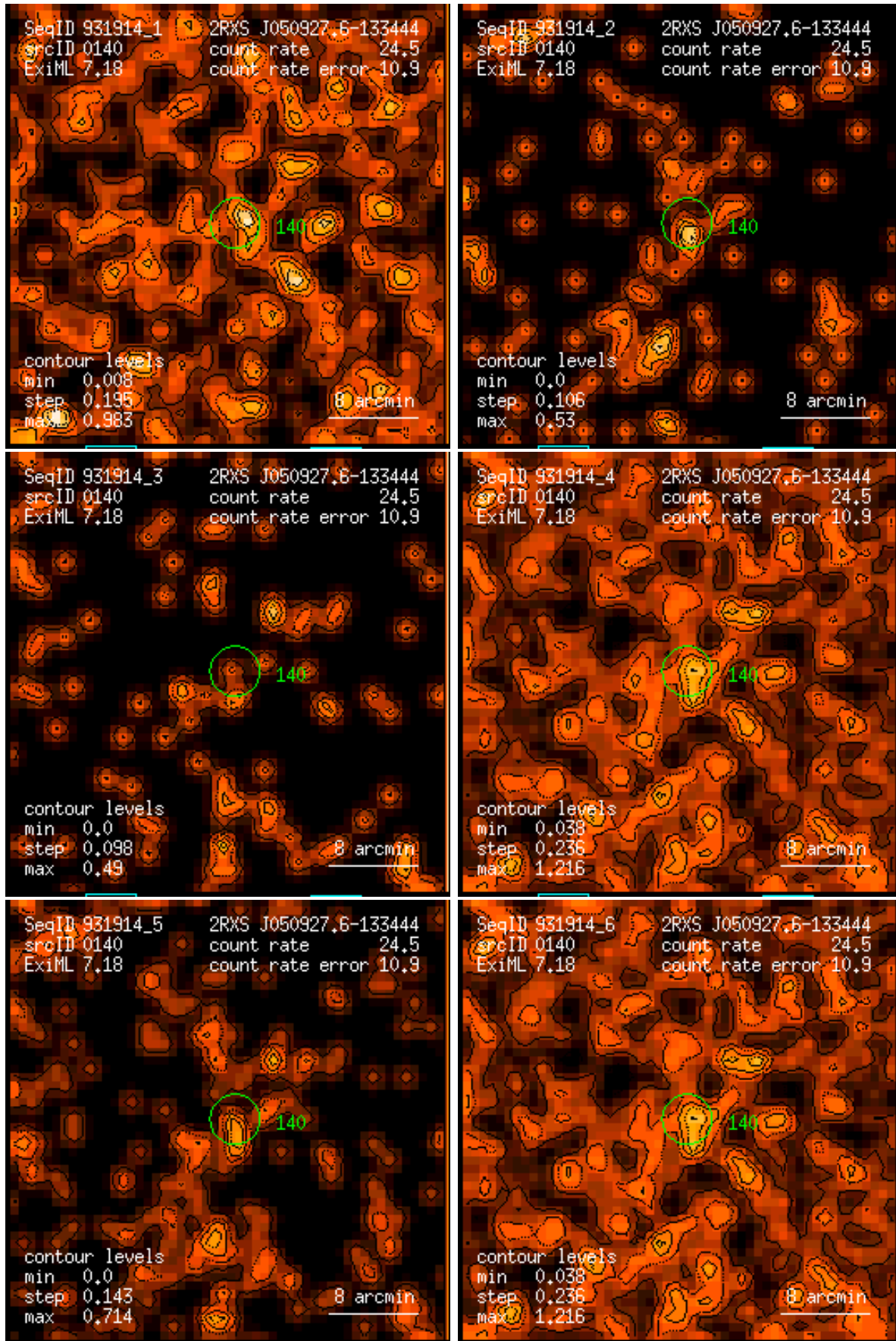
Figure 140: RASS 931914: detection 0140: band rate images, Gaussian filter: (1) PSPC channels 11 – 41, (2) 52 – 90, (3) 91 – 201, (4) 11 – 235, (5) 52 – 201, (6) 11 – 201. Broad band rates in counts/ks. Band rate contour levels in counts/ks/arcmin 2 .
