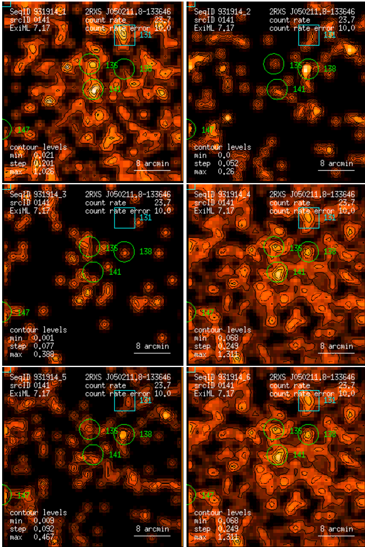
Figure 141: RASS 931914: detection 0141: band rate images, Gaussian filter: (1) PSPC channels 11 – 41, (2) 52 – 90, (3) 91 – 201, (4) 11 – 235, (5) 52 – 201, (6) 11 – 201. Broad band rates in counts/ks. Band rate contour levels in counts/ks/arcmin 2 .
