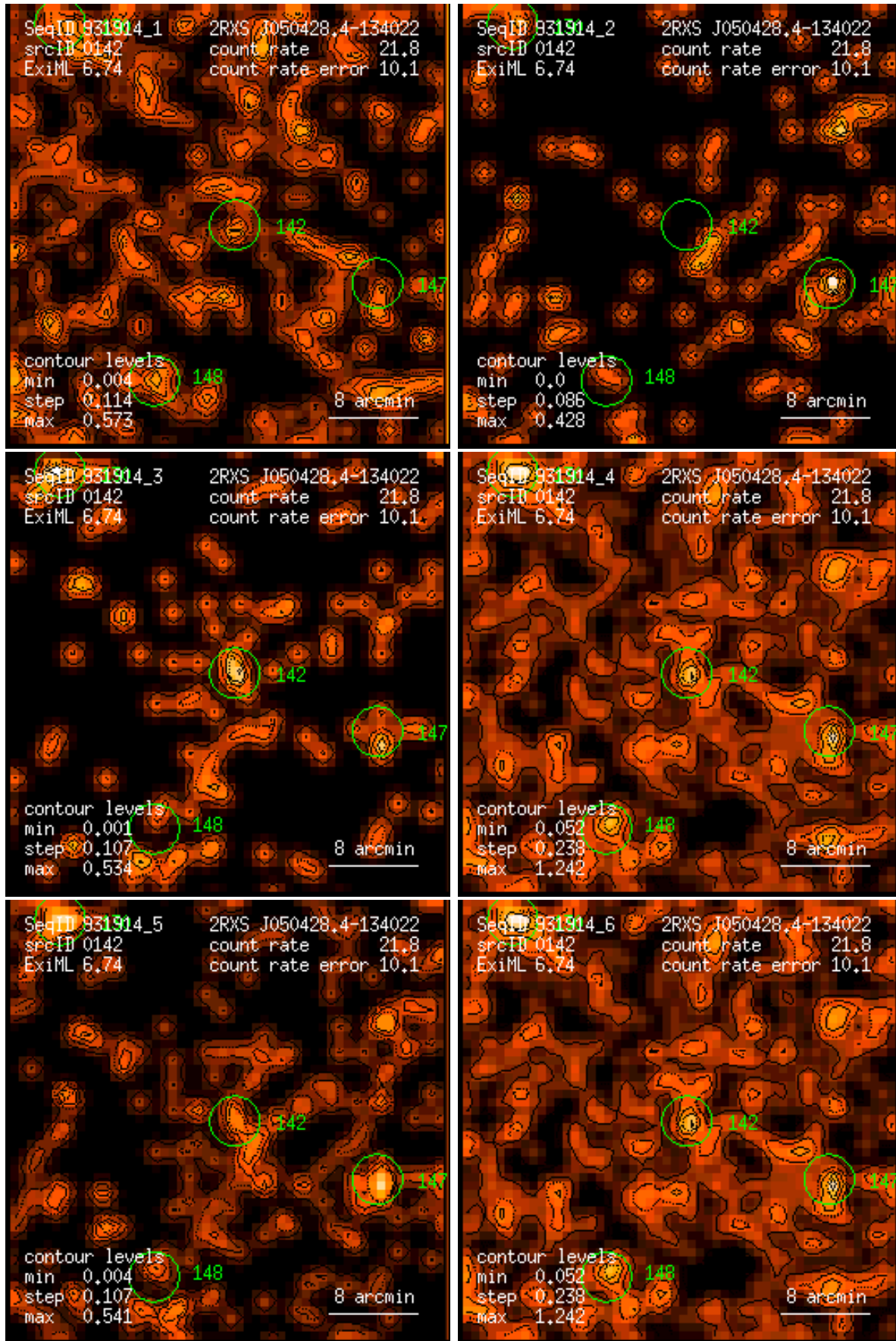
Figure 142: RASS 931914: detection 0142: band rate images, Gaussian filter: (1) PSPC channels 11 – 41, (2) 52 – 90, (3) 91 – 201, (4) 11 – 235, (5) 52 – 201, (6) 11 – 201. Broad band rates in counts/ks. Band rate contour levels in counts/ks/arcmin 2 .
