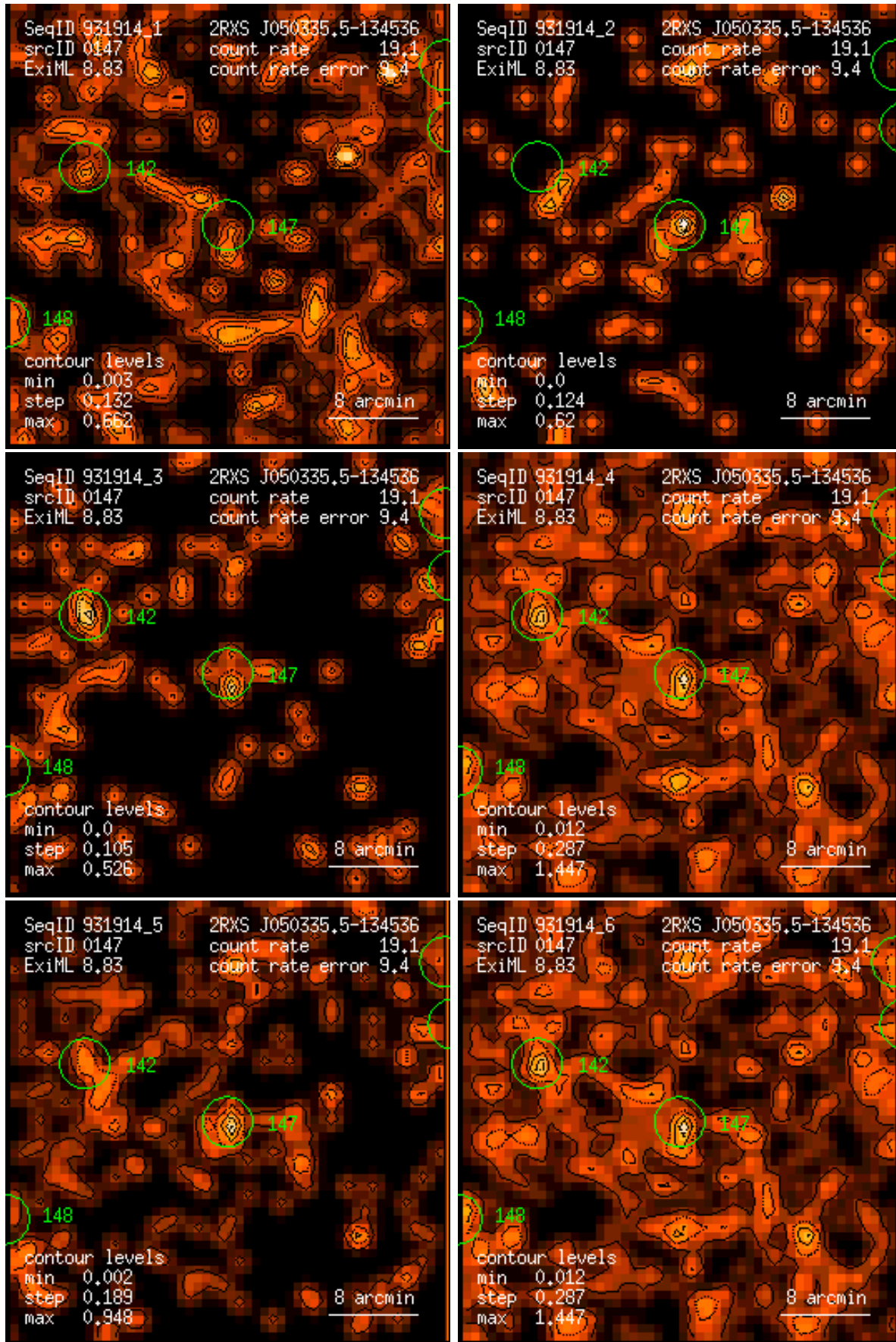
Figure 147: RASS 931914: detection 0147: band rate images, Gaussian filter: (1) PSPC channels 11 – 41, (2) 52 – 90, (3) 91 – 201, (4) 11 – 235, (5) 52 – 201, (6) 11 – 201. Broad band rates in counts/ks. Band rate contour levels in counts/ks/arcmin 2 .
