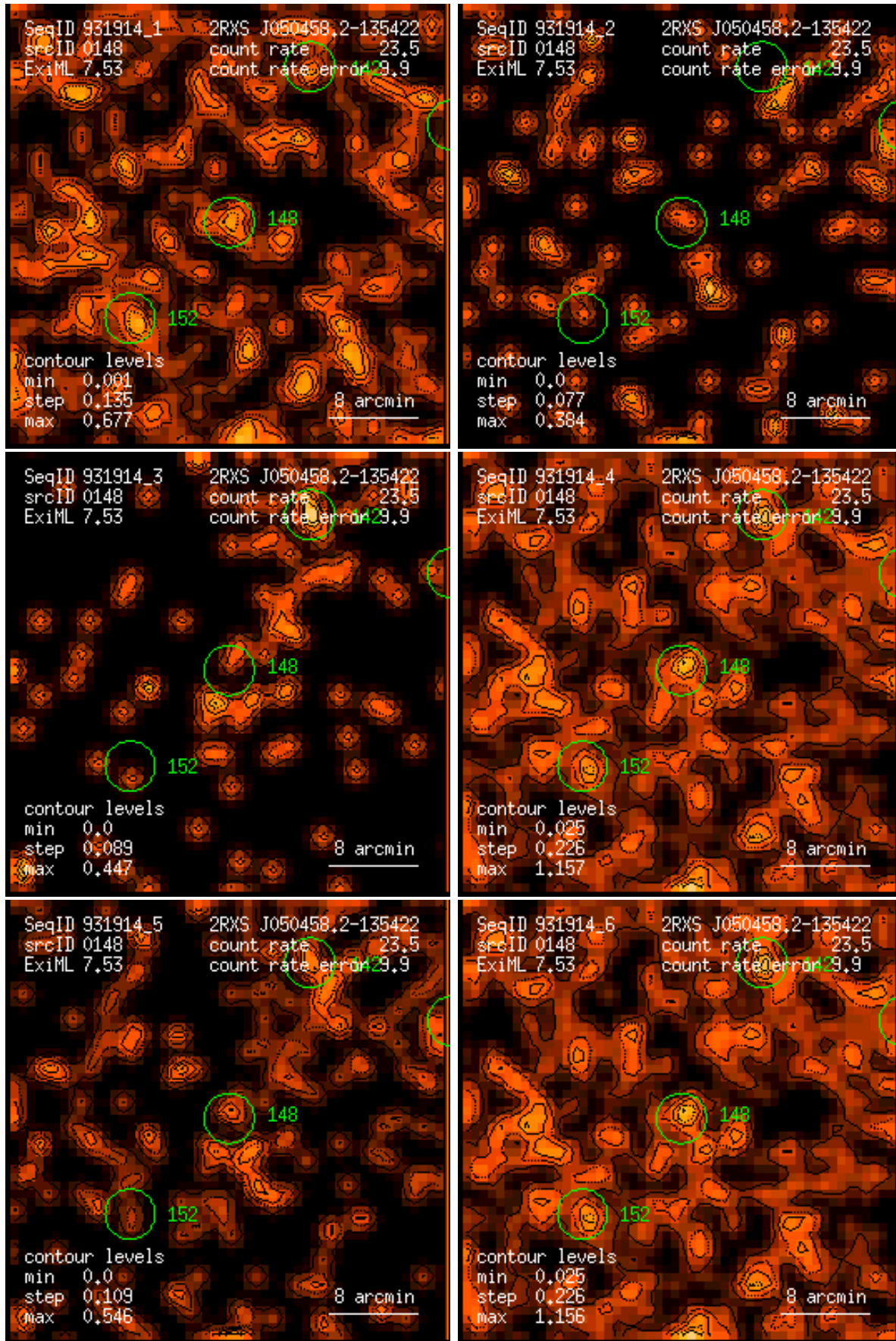
Figure 148: RASS 931914: detection 0148: band rate images, Gaussian filter: (1) PSPC channels 11 – 41, (2) 52 – 90, (3) 91 – 201, (4) 11 – 235, (5) 52 – 201, (6) 11 – 201. Broad band rates in counts/ks. Band rate contour levels in counts/ks/arcmin 2 .
