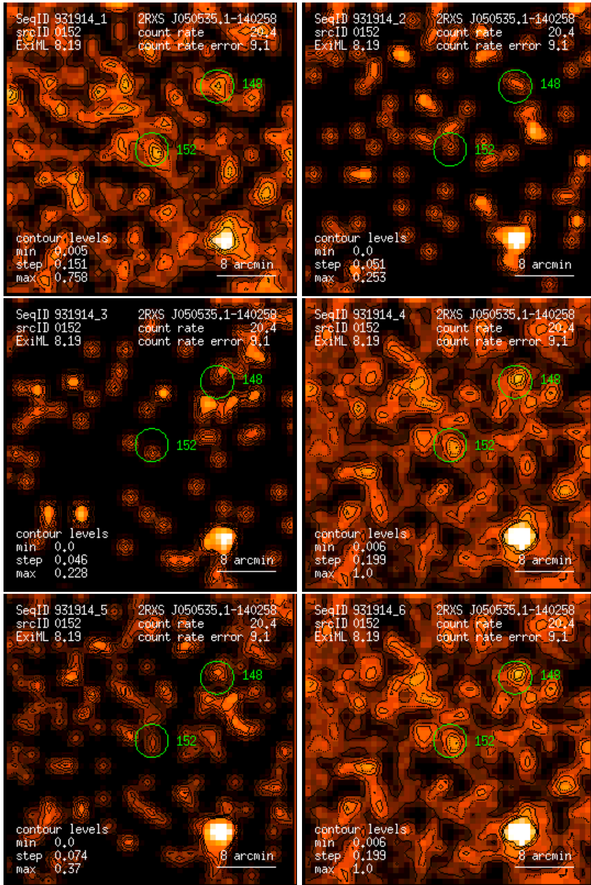
Figure 152: RASS 931914: detection 0152: band rate images, Gaussian filter: (1) PSPC channels 11 – 41, (2) 52 – 90, (3) 91 – 201, (4) 11 – 235, (5) 52 – 201, (6) 11 – 201. Broad band rates in counts/ks. Band rate contour levels in counts/ks/arcmin 2 .
