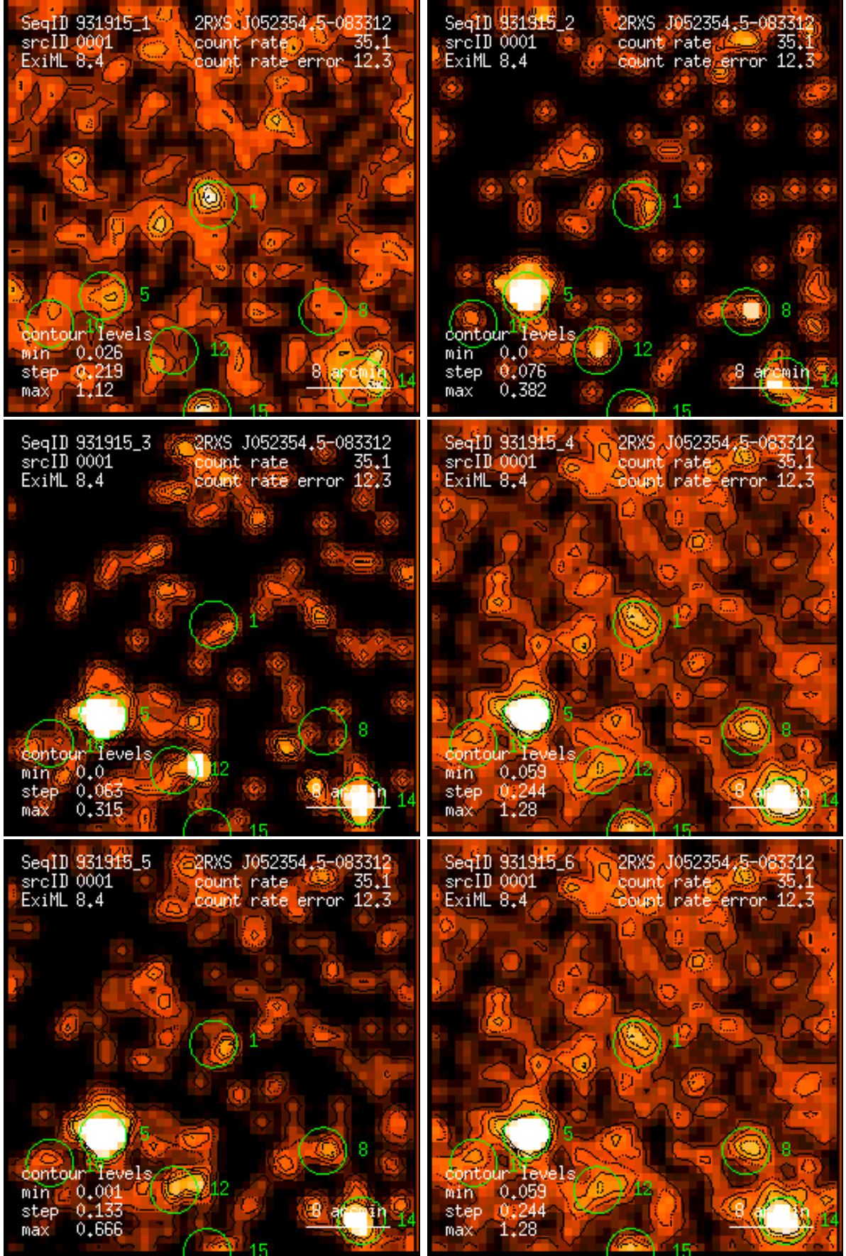
Figure 1: RASS 931915: detection 0001: band rate images, Gaussian filter: (1) PSPC channels 11 – 41, (2) 52 – 90, (3) 91 – 201, (4) 11 – 235, (5) 52 – 201, (6) 11 – 201. Broad band rates in counts/ks. Band rate contour levels in counts/ks/arcmin 2 .
