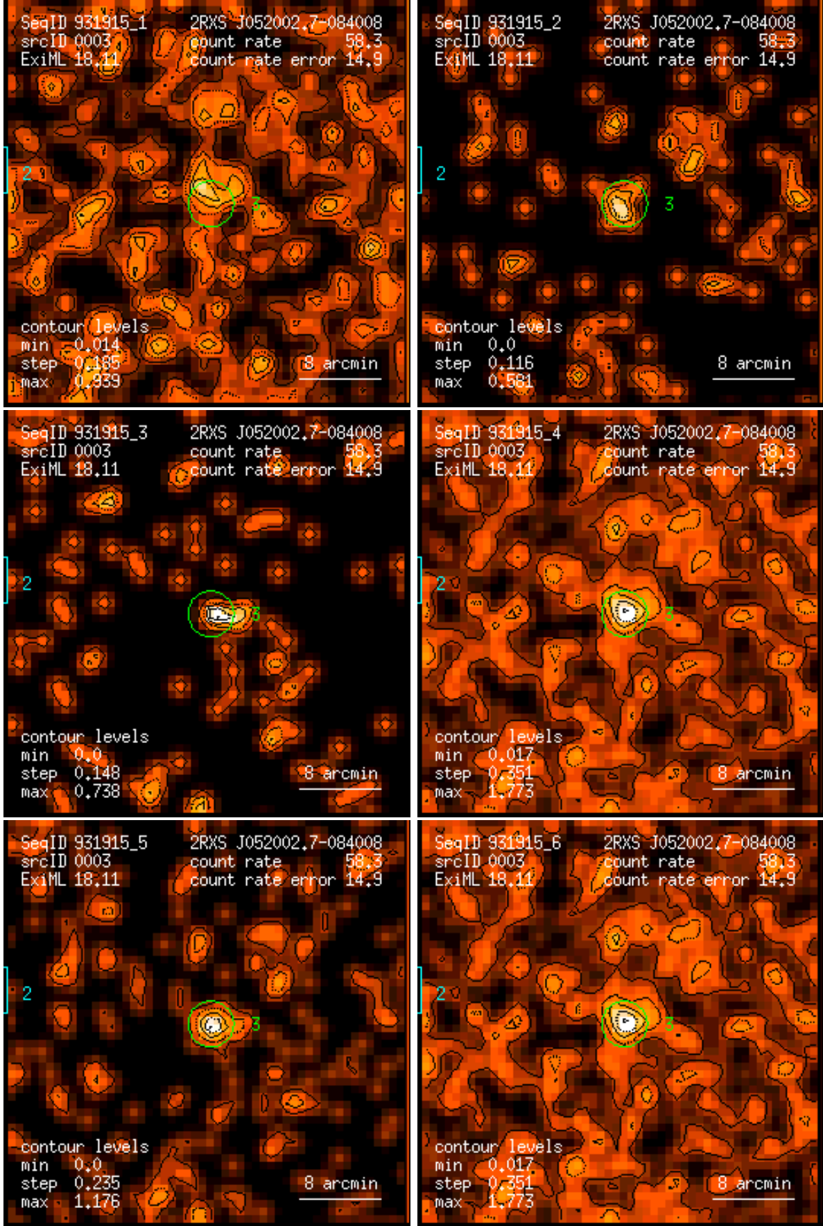
Figure 3: RASS 931915: detection 0003: band rate images, Gaussian filter: (1) PSPC channels 11 – 41, (2) 52 – 90, (3) 91 – 201, (4) 11 – 235, (5) 52 – 201, (6) 11 – 201. Broad band rates in counts/ks. Band rate contour levels in counts/ks/arcmin 2 .
