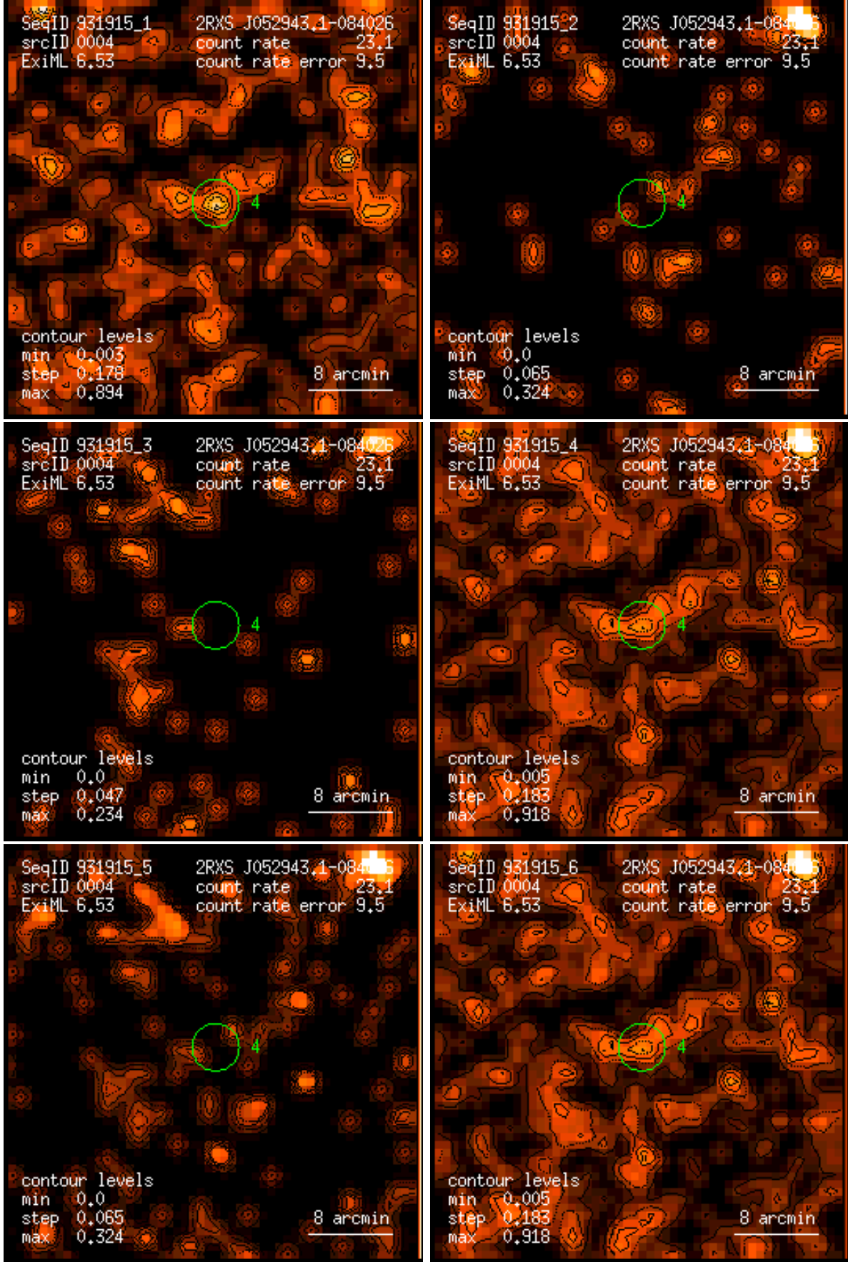
Figure 4: RASS 931915: detection 0004: band rate images, Gaussian filter: (1) PSPC channels 11 – 41, (2) 52 – 90, (3) 91 – 201, (4) 11 – 235, (5) 52 – 201, (6) 11 – 201. Broad band rates in counts/ks. Band rate contour levels in counts/ks/arcmin 2 .
