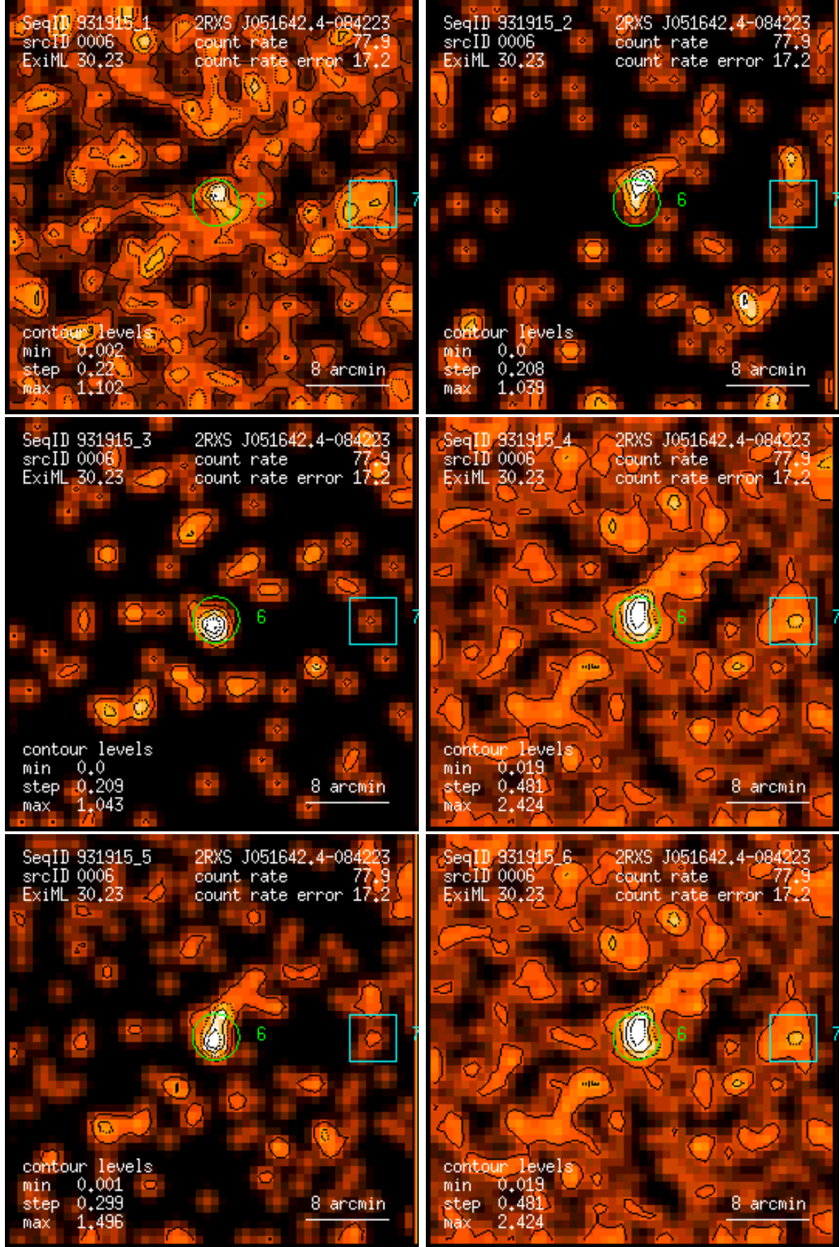
Figure 6: RASS 931915: detection 0006: band rate images, Gaussian filter: (1) PSPC channels 11 – 41, (2) 52 – 90, (3) 91 – 201, (4) 11 – 235, (5) 52 – 201, (6) 11 – 201. Broad band rates in counts/ks. Band rate contour levels in counts/ks/arcmin 2 .
