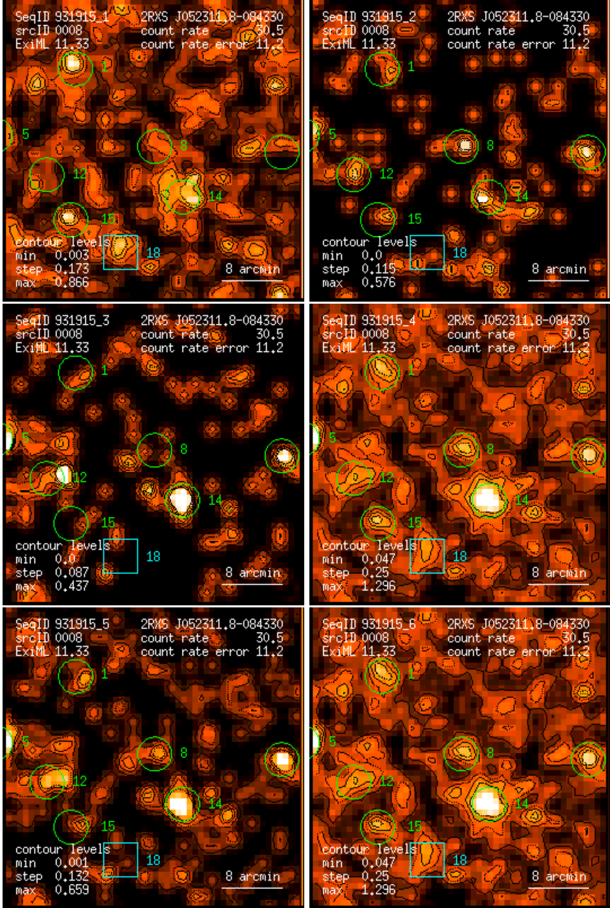
Figure 8: RASS 931915: detection 0008: band rate images, Gaussian filter: (1) PSPC channels 11 – 41, (2) 52 – 90, (3) 91 – 201, (4) 11 – 235, (5) 52 – 201, (6) 11 – 201. Broad band rates in counts/ks. Band rate contour levels in counts/ks/arcmin 2 .
