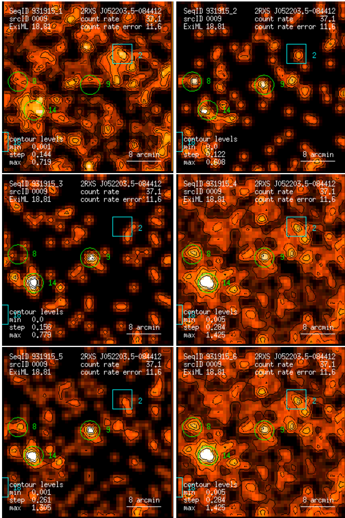
Figure 9: RASS 931915: detection 0009: band rate images, Gaussian filter: (1) PSPC channels 11 – 41, (2) 52 – 90, (3) 91 – 201, (4) 11 – 235, (5) 52 – 201, (6) 11 – 201. Broad band rates in counts/ks. Band rate contour levels in counts/ks/arcmin 2 .
