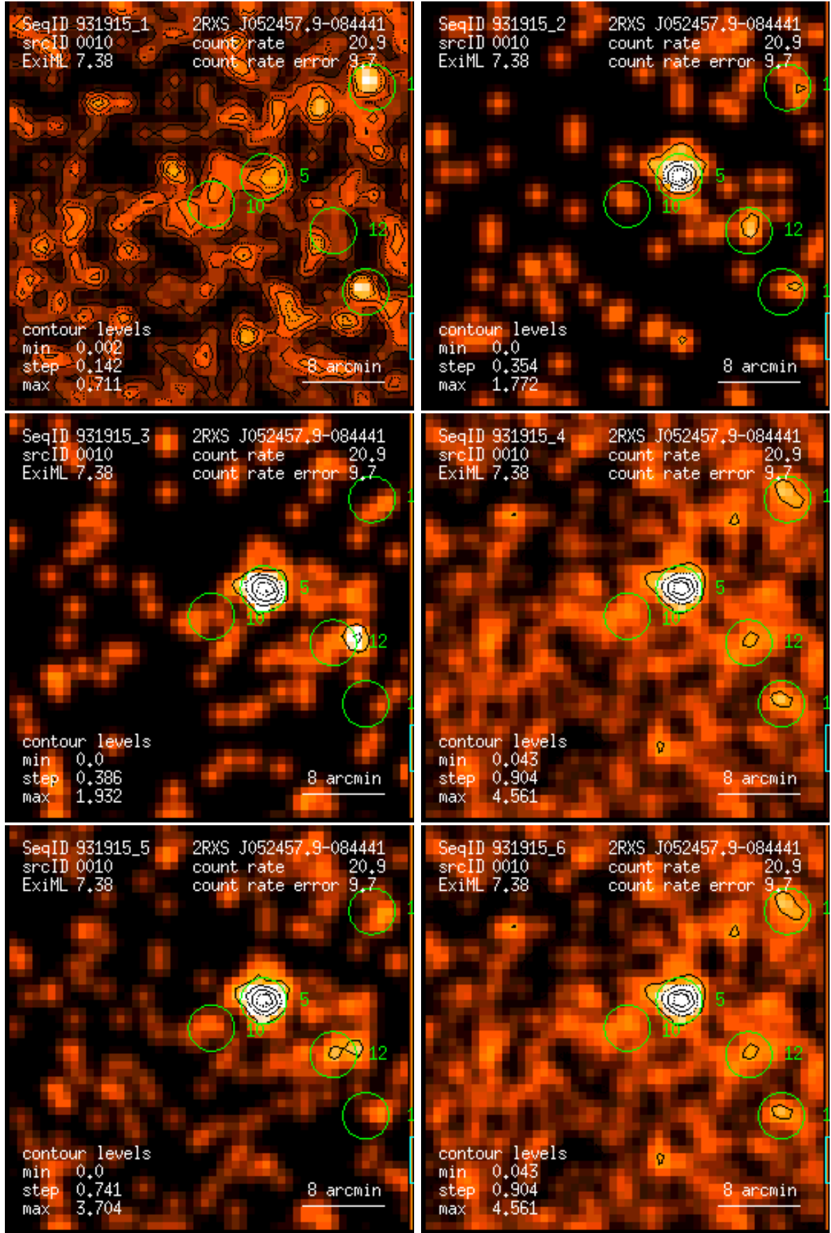
Figure 10: RASS 931915: detection 0010: band rate images, Gaussian filter: (1) PSPC channels 11 – 41, (2) 52 – 90, (3) 91 – 201, (4) 11 – 235, (5) 52 – 201, (6) 11 – 201. Broad band rates in counts/ks. Band rate contour levels in counts/ks/arcmin 2 .
